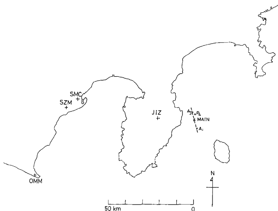
Fig. 10. The location of the observation sites and the epicenters of the mainshock and the small events used for synthesis. The mainshock is the 1980 Izu-Hanto-Toho-Oki earthquake with M=6.7 .
