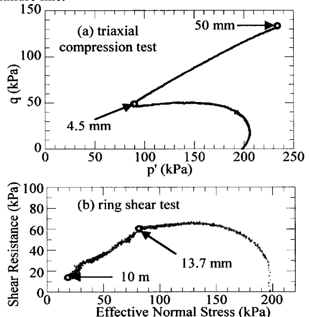
Fig. 3 Effective stress paths of loose silica sand no.8. (a) triaxial compression test ( S_{11}: e_0=1.11 ), (b) ring shear test ( S_{11}: e_0=1.10 )
