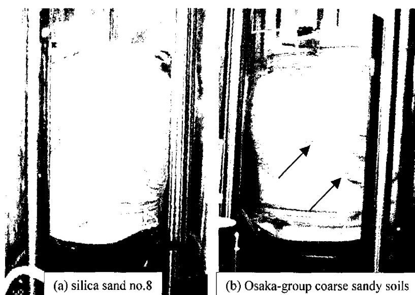
Photo. 1 Shear surfaces formed in the cylindrical dense specimens. (a) silica sand no.8 ( S_{10} : e_0 = 0.86 ), and (b) Osaka-group coarse sandy soils ( O_{18} : e_0 = 0.55 )
