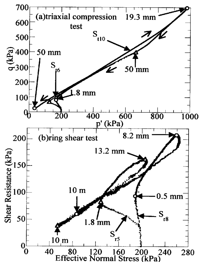
Fig. 5 Effective stress paths of medium dense and dense silica sand no.8. (a) triaxial compression test ( S_{16} : e_0 = 0.96 , S_{110} : e_0 = 0.86 ), (b) ring shear test ( S_{r5} : e_0 = 0.98 , S_{r8} : e_0 = 0.86 )
