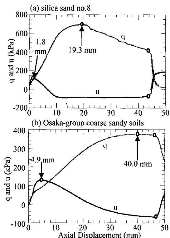
Fig. 7 Relationship of deviator stress ( q ) and pore pressure ( u ) versus axial displacement of dense specimens. (a) silica sand no.8 ( S_{10} : e_0=0.86 ), (b) Osaka-group coarse sandy soils ( O_{18} : e_0=0.55 )
