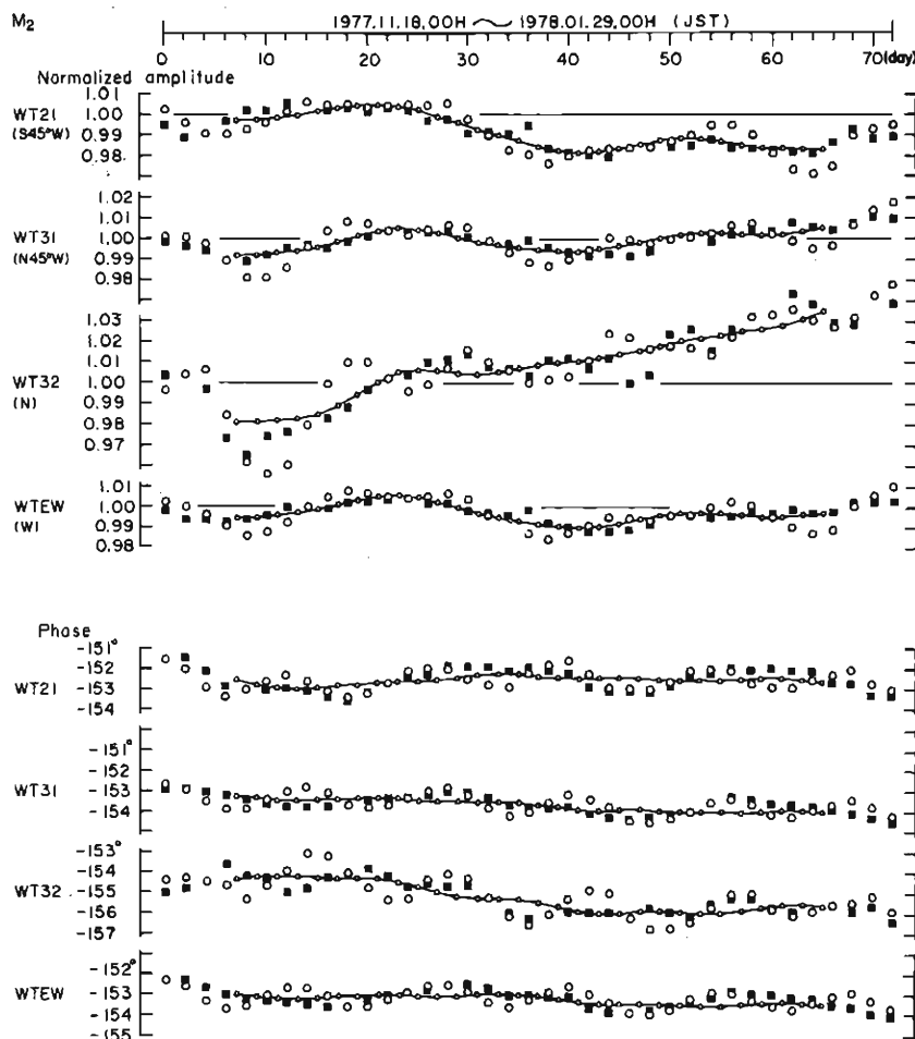
Fig. 7. Results of successive analyses for M_2 using the filtered data from Nov. 03, 00h00m, 1977 to Feb. 12, 23h00m, 1978, (JST). The solid square and large open circle show the results obtained for Cases I and II, respectively; the small open circle shows the 14-day moving average value for Case II; the phase denotes the lag when the time origin is taken at Nov. 02, 00h00m, 1977, (JST).
