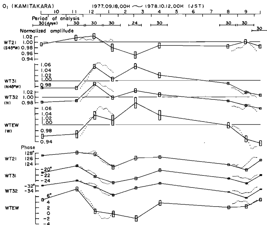
Fig. 6. Temporal variations in the amplitude and phase of O_1 . Each dot corresponds to the 14-day moving average value shown in Figs. 8 and 10 (otherwise presented as in Fig. 5).
