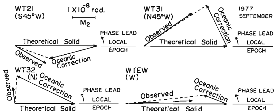
Fig. 1. Phasor plots of the M_2 tilt tide at Kamitakara. The effect of oceanic tide loading were computed by T. Tanaka.
