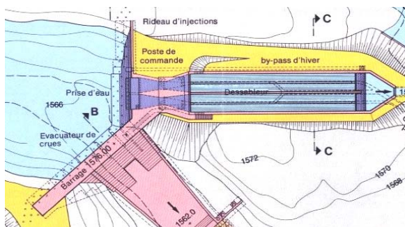
Fig. 8 Plan view of the water intake of La Fouly, part of the hydroelectric scheme of Emosson (Switzerland) (Boillat et al. 2003)
