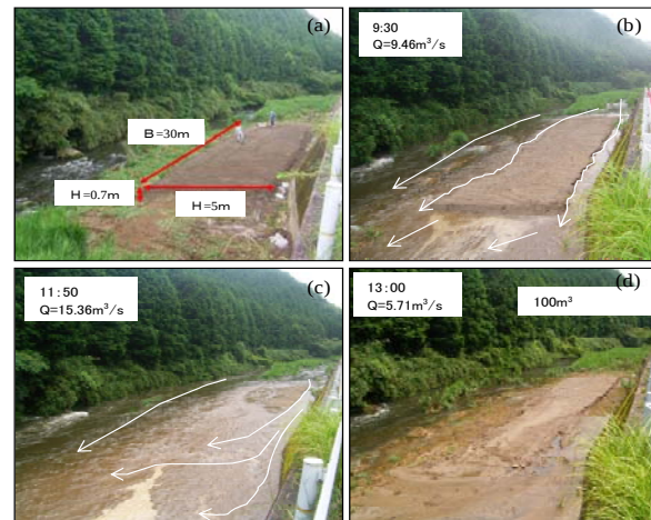
Fig. 16 Processes of erosion and deposition of the placed sediment during flood
