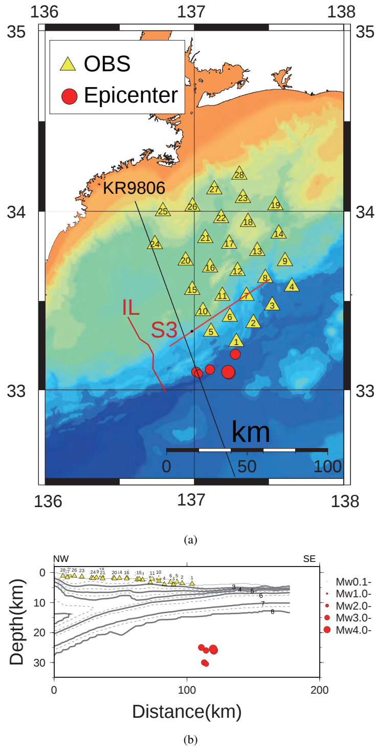
Figure. 3.9: (a) Survey area at Nankai trough. Three survey lines, KR9806, IL and S3 indicate those from Nakanishi et al. (2002), Moore et al. (2009), and Park et al. (2004) respectively. (b) The depth of OBS and earthquakes projected to the line KR9806. Background velocity contour is from refraction tomography (Nakanishi et al., 2002).
