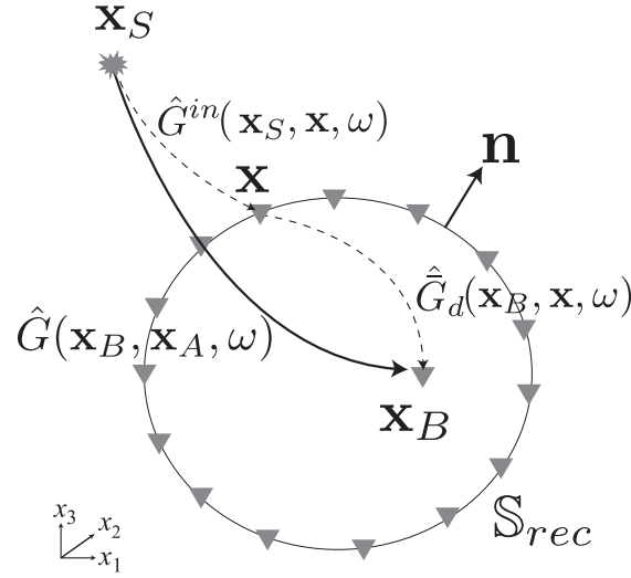
Figure. 2.5: Configuration for SI by MDD. Objective function \hat{\hat{G}}_d(\mathbf{x}_B, \mathbf{x}, \omega) is formulated as a integral along the receiver surface.
