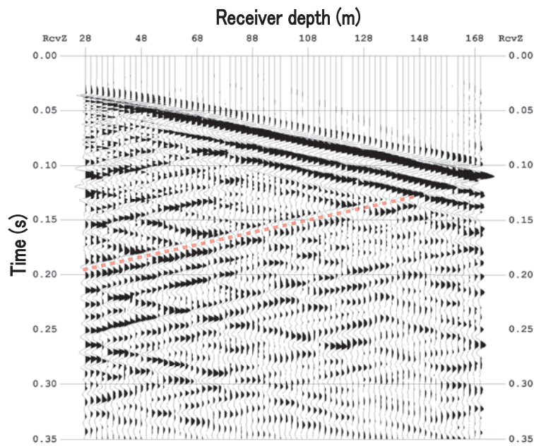
Figure. 6.9: Example of the recorded field data after preprocessing: a shot record in well-1 from the surface source at 5m distance from well-2. The pink dotted line indicates a reflection signal from a subsurface boundary.
