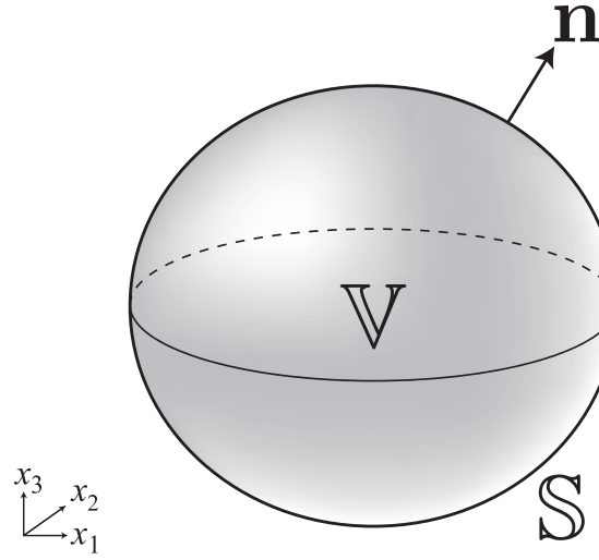
Figure. 2.1: An arbitrary inhomogeneous 3D (dissipative or lossless) acoustic media in a domain \mathbb{V} whose surface is defined as \mathbb{S} . \mathbf{n} is an outward pointing normal vector.
