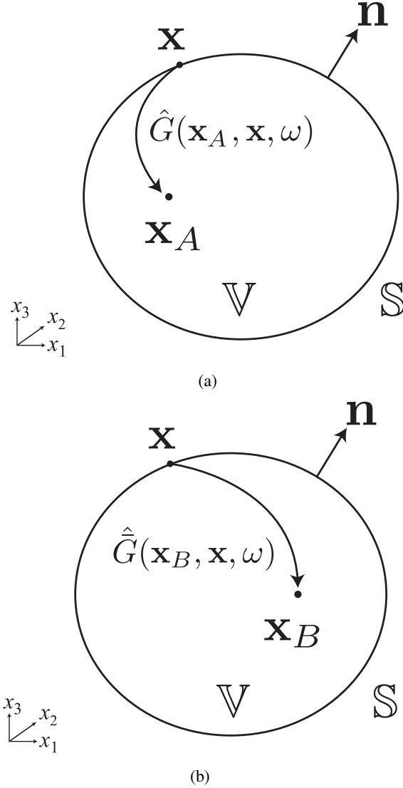
Figure. 2.2: Configuration for Correlation-type Green's function representation. (a) Impulsive source at \mathbf{x}_A for actual state (state-A). (b) Impulsive source at \mathbf{x}_B for reference state (state-B). \hat{G} or \hat{\hat{G}} indicates Green's function.
