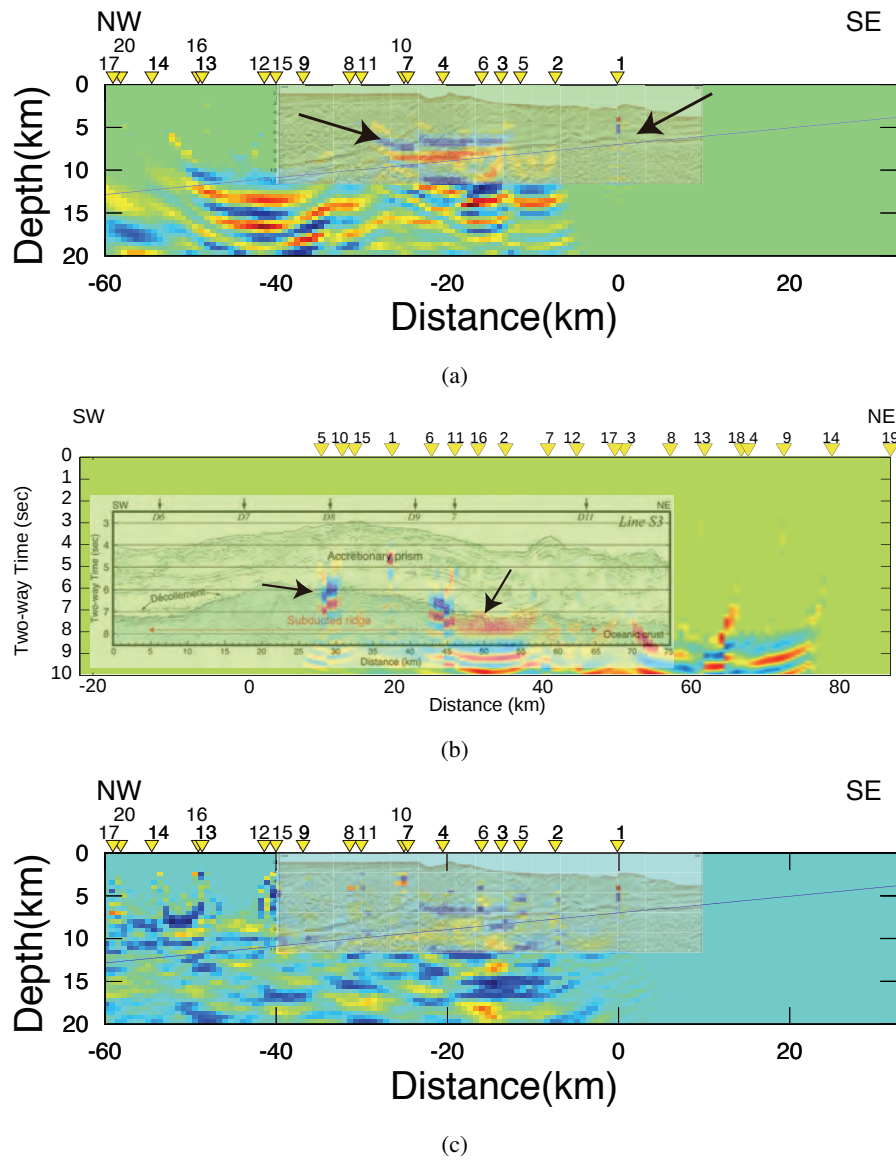
Figure. 3.13: PSDM imaging results. (a) Stacked perpendicular to Line KR9806. The seismic profile from Moore et al. (2009) is overwrapped. Arrows show the imaged upper oceanic crust boundary. (b) Stacked perpendicular to Line S3. The seismic profile from Park et al. (2004) is overwrapped. (c) Stacked perpendicular to Line KR9806 using all CC traces.
