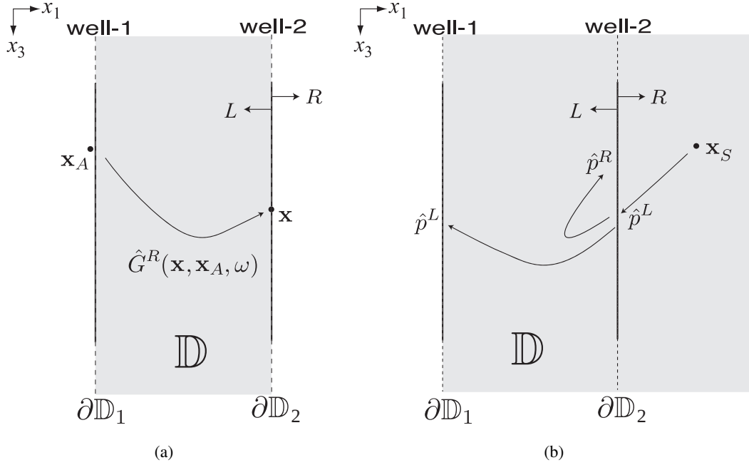
Figure. A.2: (a) Desired crosswell wavefield for state A . \mathbb{D} is a volume enclosed by the two boreholes (vertical boundaries \partial\mathbb{D}_1 and \partial\mathbb{D}_2 ) of infinite extent. \hat{G}^R(\mathbf{x}, \mathbf{x}_A, \omega) denotes the transmission response (or Green's function) from \mathbf{x}_A to \mathbf{x} . (b) Actual wavefield for state B . \hat{p}^L and \hat{p}^R represent left- and right-propagating wavefields from the source at \mathbf{x}_S . The areas shaded in gray represent heterogeneous space.
