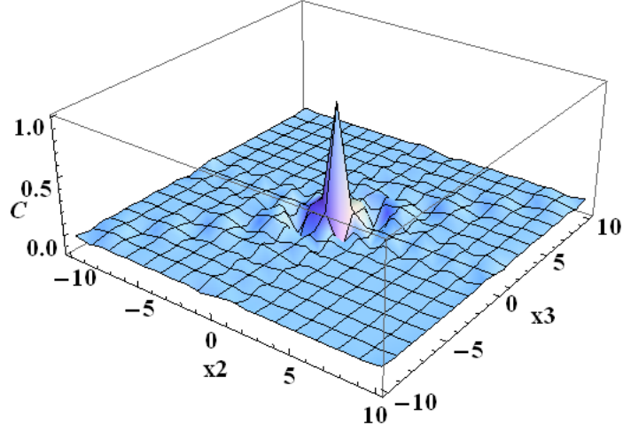
Figure 1: The solution C_{0 x_2 x_3} representing a fuzzy ring for g_1 = 1, g_2 = 2, g_3 = 1, L = 10 is plotted in the coordinate basis. The values are normalized by C_{000} . The coordinate x dual to p is defined by the discrete Fourier transformation \sum_{p=-L}^L \exp(2\pi i p x / (2L + 1)) .
