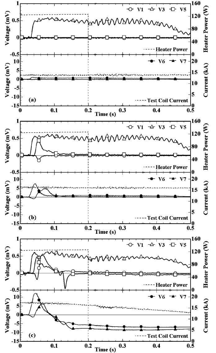
Fig. 5. Typical waveforms of the voltages between each taps and the test coil current for the liquid He temperature of 2.0 K. (a) B = 6.35 T, I = 13.8 kA, (b) B = 6.48 T, I = 16.3 kA, (c) B = 6.57 T, I = 17.4 kA.
