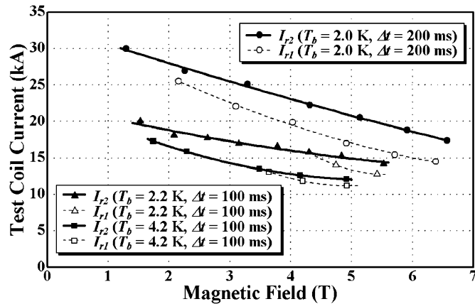
Fig. 7. Stability limit currents for the LHD test coil as a function of the magnetic flux density for the different liquid He temperature. For all the tests, input heater power was 125 W.
