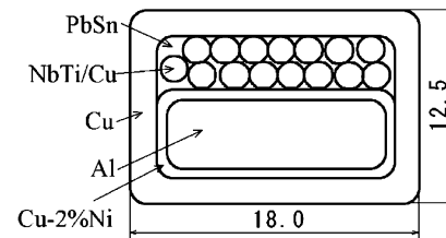
Fig. 1. Cross-sectional view of the LHD conductor.
