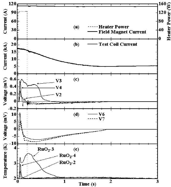
Fig. 6. Overall trends of the test results belong to Group III. T_b = 2.0 K, B = 6.57 T, I = 17.4 kA, \Delta t = 200 ms. (a) Field magnet current, (b) test coil current, (c) voltages between each taps, (d) voltages between each turns, (e) temperatures of the \text{RuO}_2 thermometers.
