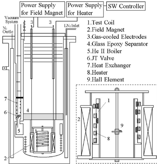
Fig. 2. Schematic of the experimental setup.
