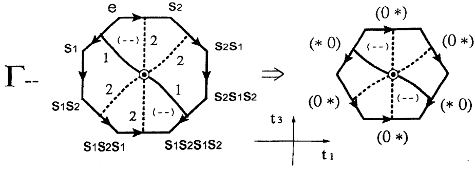
FIGURE 4. The C_2 Toda lattice in the nilpotent limit. The Painlevé divisors \mathcal{D}_{\{1\}} and \mathcal{D}_{\{2\}} are shown as the solid and the dashed curves, respectively. Four boundaries marked by (0*) intersecting with \mathcal{D}_{\{2\}} in the right hexagon should be identified with the orientation given by the direction of the flow. Two other boundaries marked by (*0) are also identified. Then the compact variety \tilde{Z}(0)_{\mathbb{R}} is orientable and singular.
