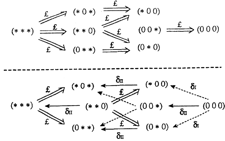
FIGURE 8. The graph \mathcal{G}_{A_3}^L and its decomposition into two identical subgraphs giving rise to the double chain complex structure. The direction of the arrows \delta_{II} is as in Figure 7.
