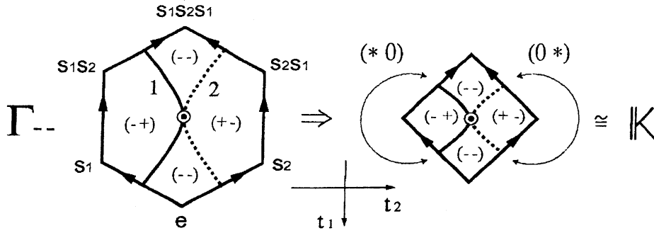
FIGURE 2. The \mathfrak{sl}(3, \mathbb{R}) Toda lattice in the nilpotent limit. The Painlevé divisors \mathcal{D}_{\{1\}} and \mathcal{D}_{\{2\}} are shown as the solid and the dashed curves, respectively. In the limit, the left two sides of the square are identified, so are the right two sides. The compact variety is then homologous to the Klein bottle \mathbb{K} .
