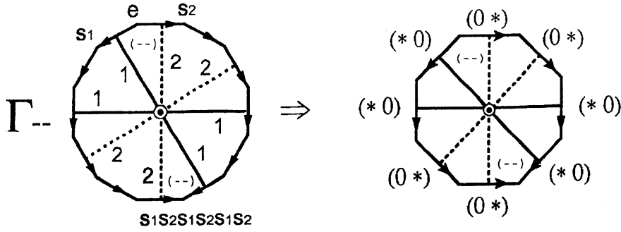
FIGURE 5. The G_2 Toda lattice in the nilpotent limit. The Painlevé divisors \mathcal{D}_{\{1\}} and \mathcal{D}_{\{2\}} are shown as the solid and the dashed curves, respectively.
