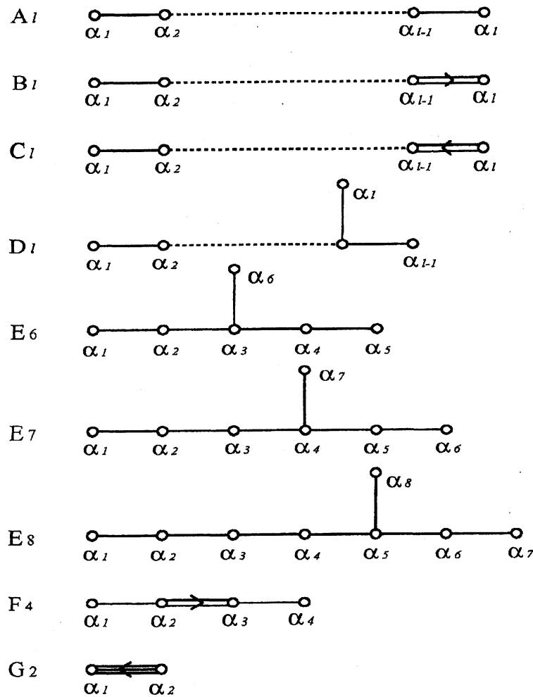
FIGURE 9. The Dynkin diagrams for simple Lie algebras and the labeling on the simple roots
