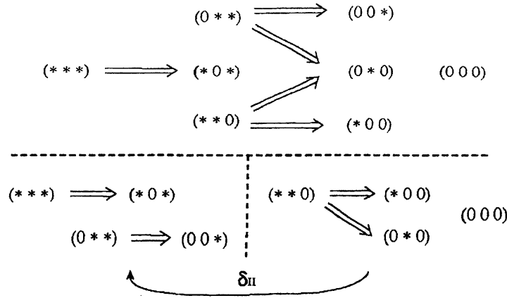
FIGURE 7. The graph \mathcal{G}_{A_n} and its decomposition into two subgraphs giving rise to the double chain complex structure. One in the bottom right is a graph \mathcal{G}_{A_2} for \{\langle J \rangle = (\cdot \cdot 0)\} . The bottom left is a graph \mathcal{G}_{A_2}^C for \{\langle J \rangle = (\cdot \cdot *)\} .
