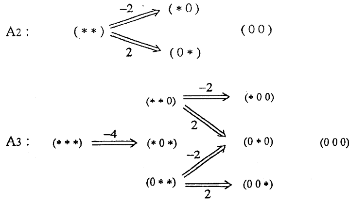
FIGURE 3. The weighted graphs \mathcal{G}_{A_l} for l = 2, 3 .
