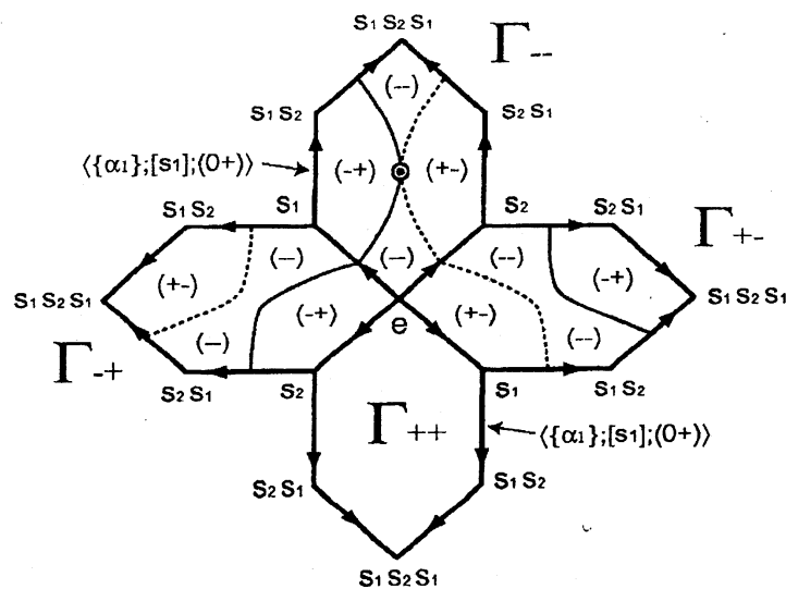
FIGURE 1. The hexagons \Gamma_\epsilon and the Painlevé divisors for \mathfrak{sl}(3, \mathbb{R}) Toda lattice. The Painlevé divisors are indicated with a solid curve for \mathcal{D}_{\{1\}} and with a dashed curve for \mathcal{D}_{\{2\}} . The double circle at the center of the \Gamma_{--} polytope is \mathcal{D}_\Pi . The arrows in the boundaries of \Gamma_\epsilon 's show the flow direction of the Toda orbit.
