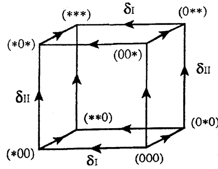
FIGURE 6. Double chain complex structure in \mathcal{C}^* for A_3 . Top of the cube corresponds to \mathcal{C}^*(\mathcal{L}) for A_2 and the bottom to a chain complex \mathcal{C}^* for A_2 .
