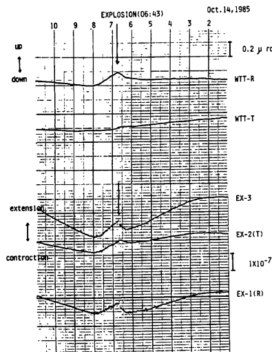
Fig. 3 A typical example of the tilt change and the strain associated with an explosive eruption.
