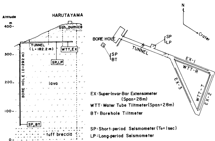
Fig. 2 Geological structure of Harutayama lava dome on the vertical cross-section and the arrangement of the instruments in the tunnel and the borehole.
