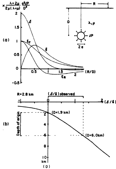
Fig. 9 (a) Distribution of the tilt and the strains calculated according to Mogi's model and (b) The relation between the depth of origin and the ratio of the dilatation to the tilt at a distance of 2.8 kilometers. Notations \delta , \epsilon_R , \epsilon_T and \Delta denote the tilt, the radial strain, the tangential strain and the dilatation, respectively.
