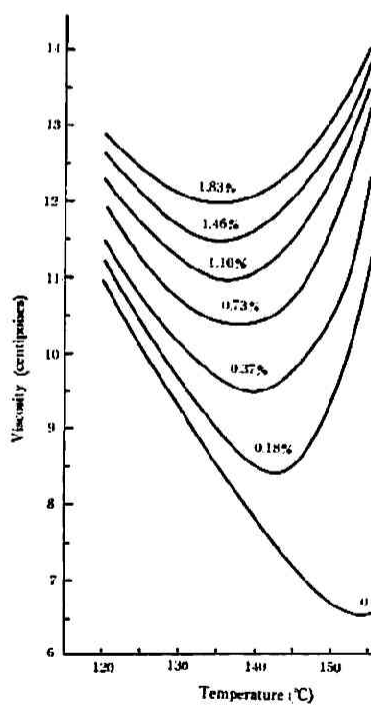
Fig. 5 Effect of S_2Cl_2 on the viscosities of sulfur
