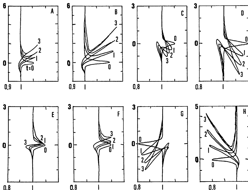
Fig. 2 Evolution of vorticity front. (Arbitrary scaling for time stepping.)
