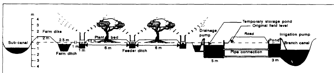
Fig. 2 A Typical Farm Structure and Necessary Infrastructure Setup of Citrus Garden
