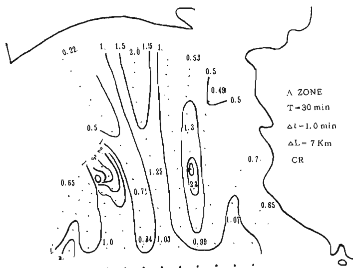
Fig. 3 Wave height distribution of simulated Chilean Tsunami in 1960 by a computer
