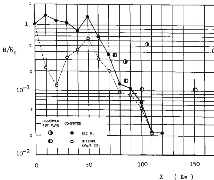
Fig. 5 Transformation of simulated tsunami in wave height by manual drawing along the coast from Pacific Ocean to Osaka Bay
