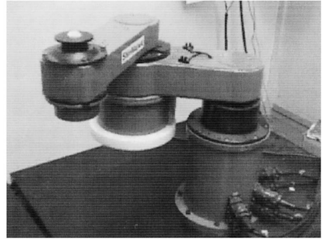
Fig. 2. Two-link manipulator.
