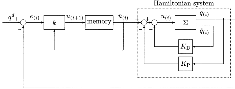
Fig. 1. Iterative learning control of mechanical systems.
