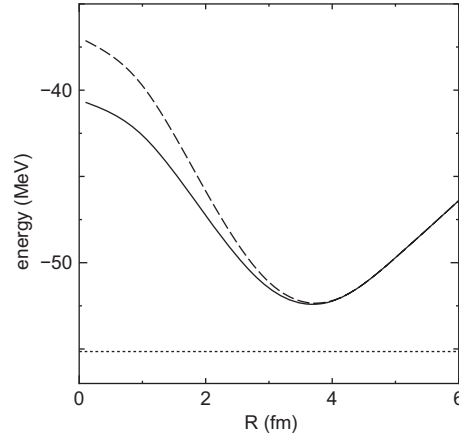
Fig. 2. The 0^+ energy curves of ^8\text{Be} . The dashed curve is for \alpha - \alpha as a function of parameter R representing the distance between two \alpha 's, and in the solid line, change into quasi-clusters is allowed. The optimal \Lambda value which gives the lowest energy is selected for each R value in the solid line. The dotted line at -55.14 MeV shows the threshold energy of two \alpha clusters.
