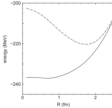
Fig. 8. The 0^+ energy curves of ^{28}\text{Si} with the pentagon shape as functions of the distance parameter R . Five quasi-clusters are placed with a pentagon shape at the distance of R from the origin and two \alpha clusters are set on the vertical axis at R/2 and -R/2 , as in Fig. 6(a). The dashed line is the case of \Lambda = 0 for the quasi-clusters, which is equivalent to \alpha clusters, and for the solid line, the optimal \Lambda value giving the lowest energy is chosen for each R .
