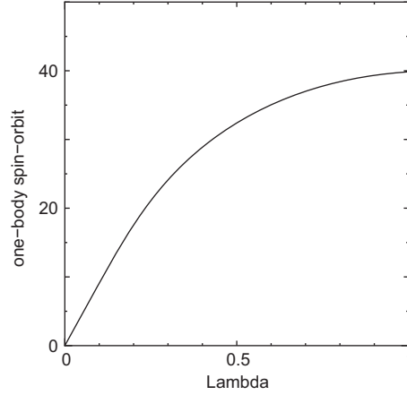
Fig. 17. The expectation value of the one-body spin-orbit operator ( \sum_i \vec{l}_i \cdot \vec{s}_i ) for ^{100}\text{Sn} in units of \hbar^2 . The \Lambda value is changed from 0 to 1.
