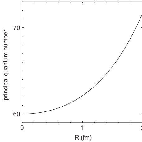
Fig. 11. The expectation value of the principal quantum number of the harmonic oscillator for ^{40}\text{Ca} as a function of the distance parameter R between each \alpha cluster and the origin.
