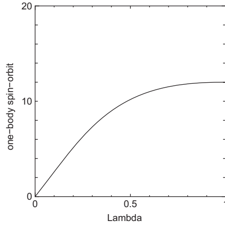
Fig. 7. The expectation value of the one-body spin-orbit operator ( \sum_i \vec{l}_i \cdot \vec{s}_i ) for ^{28}\text{Si} in units of \hbar^2 . The five quasi- \alpha clusters form a pentagon shape on the xz -plane with the distance R = 0.01 fm, and two \alpha clusters are set on the y -axis at R/2 and -R/2 as in Fig. 6(a). The \Lambda value is changed from 0 to 1.
