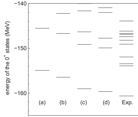
Fig. 5. The 0^+ energy levels of ^{20}\text{Ne} : (a) obtained with the ^{16}\text{O}+\alpha model space; (b) obtained by coupling (a) with the basis states, where \alpha is changed to a quasi-cluster; (c) ^{12}\text{C}+\alpha+\alpha states are coupled to (b), and the ^{12}\text{C} part is an equilateral triangular shape of three \alpha clusters; (d) the breaking effect of \alpha clusters in ^{12}\text{C} is taken into account by introducing the \Lambda parameter for ^{12}\text{C} . “Exp.” stands for the observed 0^+ states.
