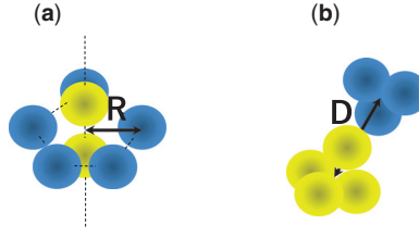
Fig. 6. (color online) Schematic figures for ^{28}\text{Si} . Spheres represent \alpha clusters, and blue ones are changed into quasi-clusters. (a) Five quasi-cluster are placed in a pentagon shape on a plane at a distance R from the origin, and two \alpha clusters are set on the vertical axis at R/2 and -R/2 . (b) ^{12}\text{C}+^{16}\text{O} shape. The parameter D is set for the distance between ^{12}\text{C} and ^{16}\text{O} . ^{12}\text{C} consists of three quasi-clusters and ^{16}\text{O} consists of four \alpha clusters with a tetrahedron shape.
