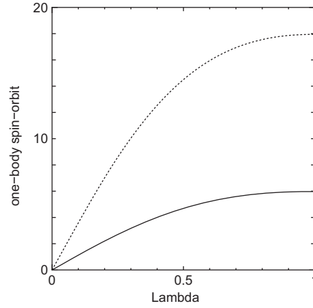
Fig. 12. The expectation value of the one-body spin-orbit operator ( \sum_i \vec{l}_i \cdot \vec{s}_i ) for ^{44}\text{Ti} in units of \hbar^2 (solid line). One quasi-cluster is placed on the x -axis at a distance of R = 0.1 fm from the ^{40}\text{Ca} core, and \Lambda is changed from 0 to 1. The value for ^{52}\text{Fe} is shown by the dotted line, and the distance parameter R for the three quasi-clusters is set to 0.25 fm. For the ^{40}\text{Ca} core part, R in Fig. 10 is set to 0.01 fm, smaller than the value for the quasi-cluster(s).
