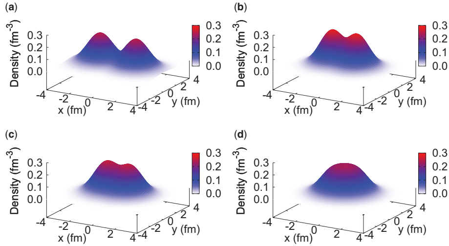
Fig. 1. (color online) Density plots of ^8\text{Be} on the z = 0 plane ( xy -plane) as a function of R and \Lambda . (a) R = 3 fm, \Lambda = 0 ; (b) R = 0.01 fm, \Lambda = 0 ; (c) R = 0.01 fm, \Lambda = 0.5 ; and (d) R = 0.01 fm, \Lambda = 1 . The integrated density is normalized to the number of nucleons.
