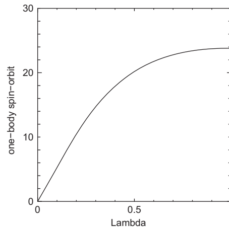
Fig. 15. The expectation value of the one-body spin-orbit operator ( \sum_i \vec{l}_i \cdot \vec{s}_i ) for ^{56}\text{Ni} in units of \hbar^2 . The \Lambda value is changed from 0 to 1.
