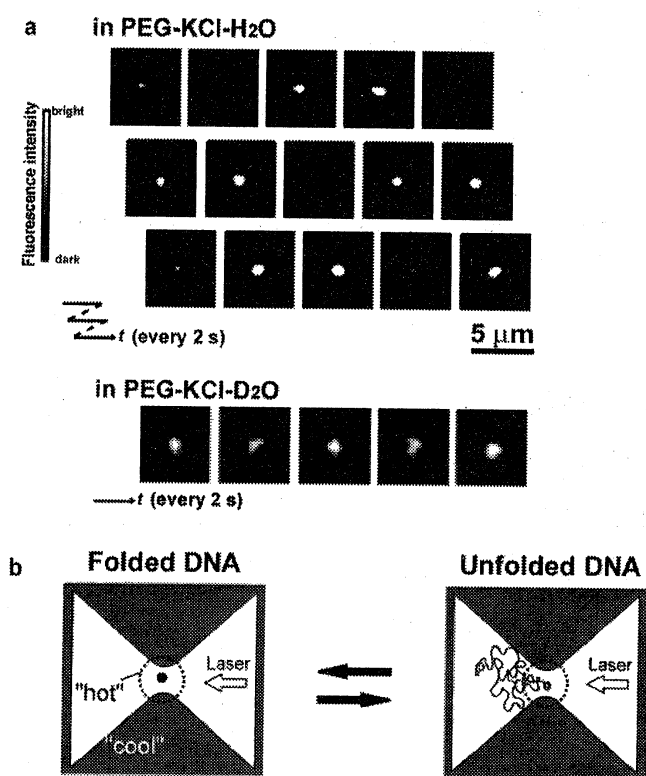
Fig. 1 Rhythmic folding/unfolding transition between the folded and unfolded states in single T4DNA molecule. (a) Time series of fluorescence image of a T4DNA molecule under the illumination of a focused CW Nd:YAG laser (1064 nm). (b) Schematic representation of rhythmic conformational change.
