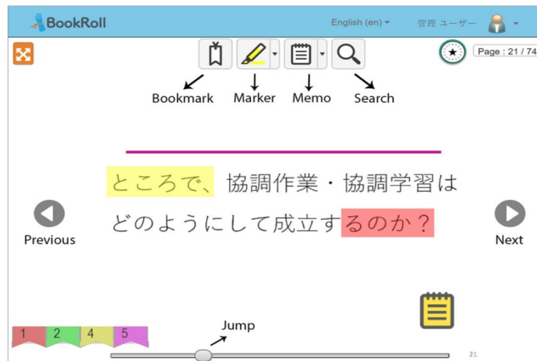
Figure 2. Screenshot of the BookRoll system's user interface
