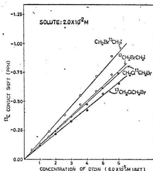
Figure 4. Observed ^{13}\text{C} contact shift plotted against the concentration of DTBN for 1,2-dihaloethanes.
