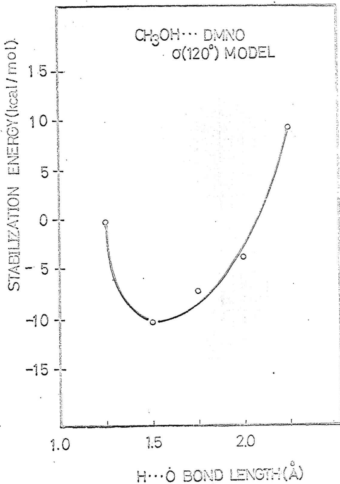
Figure 11. INDO MO stabilization energy curves plotted against the hydrogen bond length ( \sigma(120^\circ) model).
