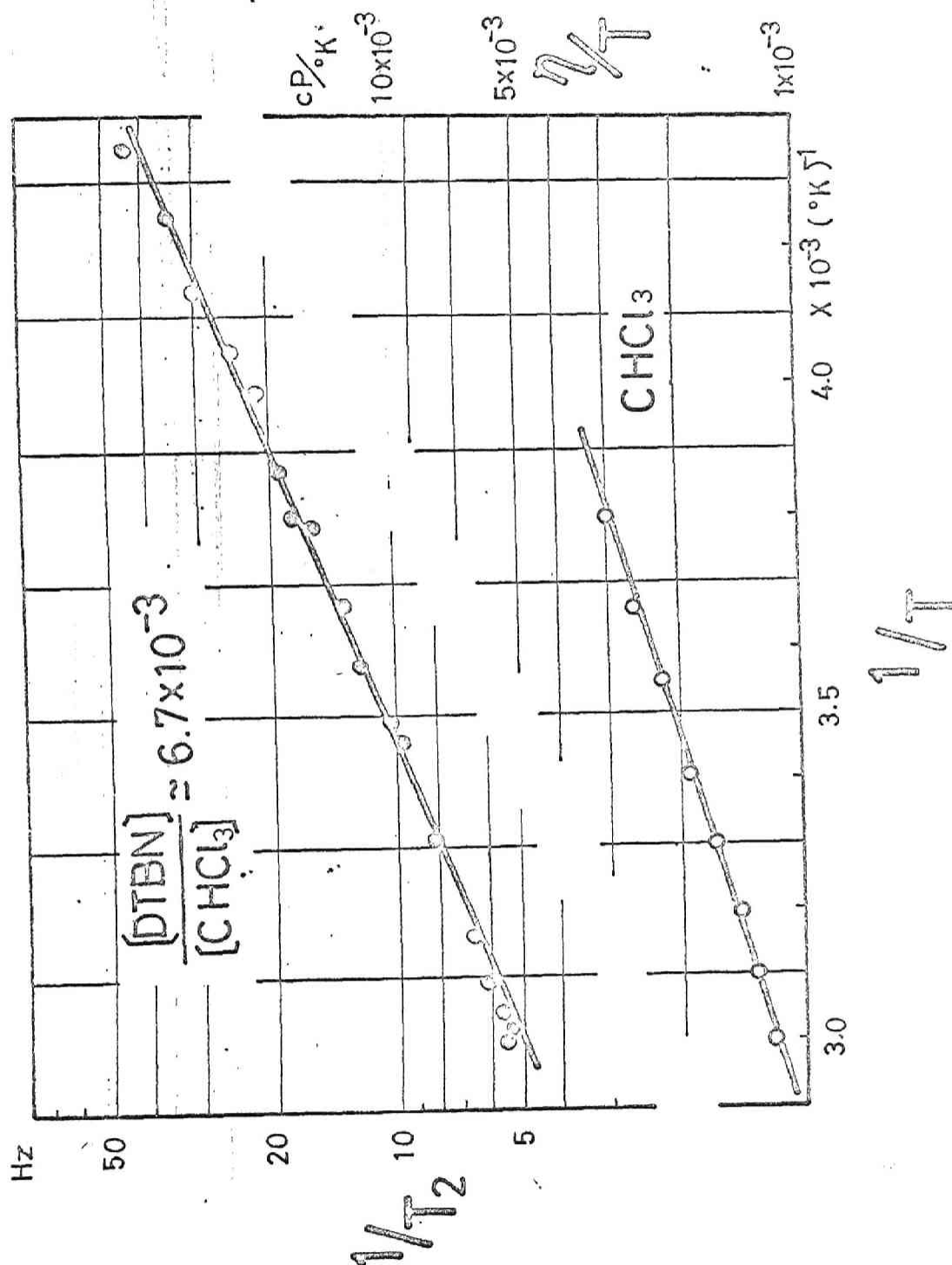
Figure 3. Temperature dependence of relaxation time and viscosity for \text{CHCl}_3
