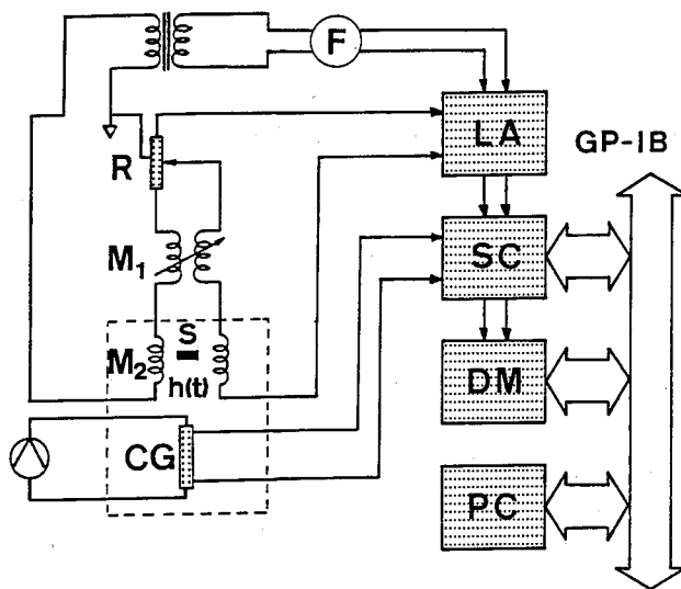
Fig. 3. Schematic diagram of the measuring system. M_1 : Variable standard mutual inductance, M_2 : Cryostat coil, R : Phase-shift potentiometer, S : Sample, CG : Carbon-glass thermometer, F : Function generator, LA : Two-phase lock-in analyzer, SC : Universal scanner, DM : Computing digital multimeter, PC : Personal computer.
