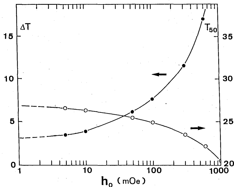
Fig. 8. Transition width \Delta T (10–90%) and the midpoint temperature T_{50} versus h_0 , where f=132 Hz. Both \Delta T and T_{50} are in unit of Kelvin.
