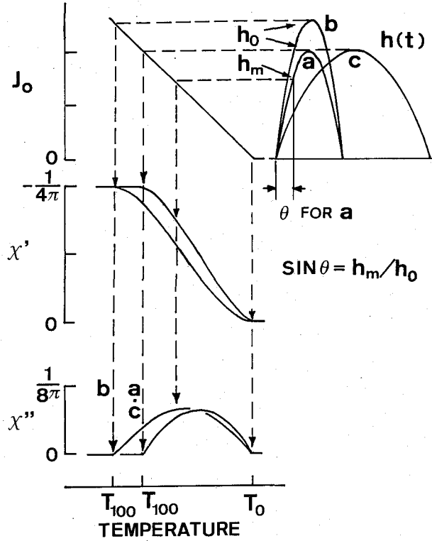
Fig. 11. Calculated \chi' and \chi'' for three different ac field, h(t) = h_0 \sin 2\pi ft . J_0 is for the Josephson tunnel junction. (a) and (b) have different h_0 , but f is the same. (a) and (c) have the same h_0 , but f is different. The transition is completed when h_m = h_0 ( \theta = \pi/2 ). Note that the completion temperature T_{100} is lowered for higher h_0 .
