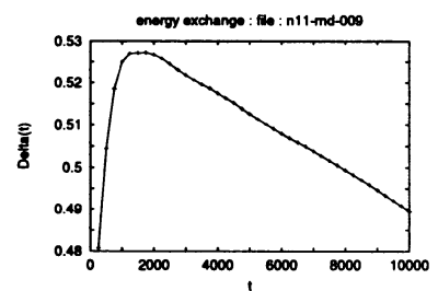
(c) Temporal evolution of \Delta(t) for 0 \leq t \leq 10000
