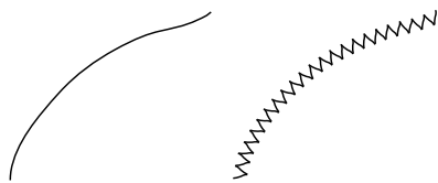
Figure 2: C^0 -close Legendrian approximation of a curve.
