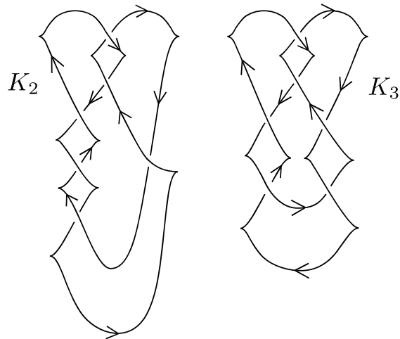
Figure 6: the Chekanov knots.
