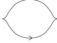
Figure 7: A Legendrian unknot with tb = -1 .
