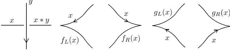
Figure 10: Relations at crossings and cusps (2).
