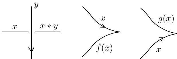
Figure 9: Relations at crossings and cusps (1).
