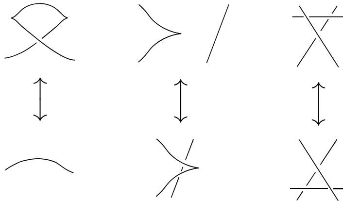
Figure 4: Legendrian Reidemeister moves.
