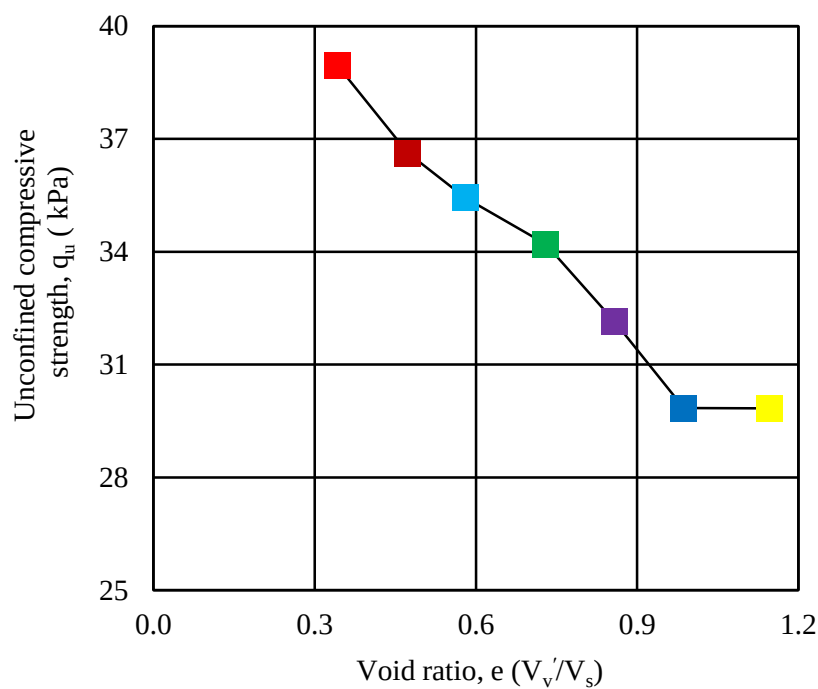
Fig. 3.36 UCS value versus void ratio ( V_v'/V_s )
