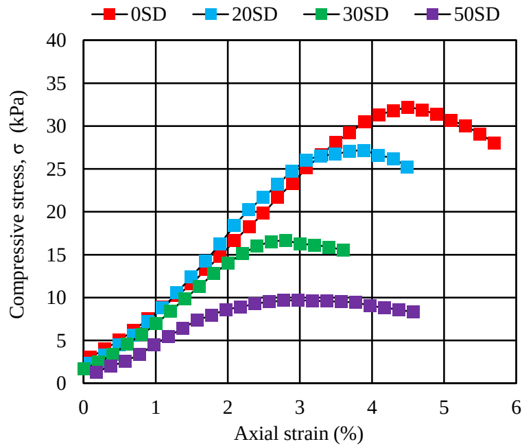
Fig. 4.4 Stress-strain relationship for various percentages of simulated decomposition for basic sample 8W
