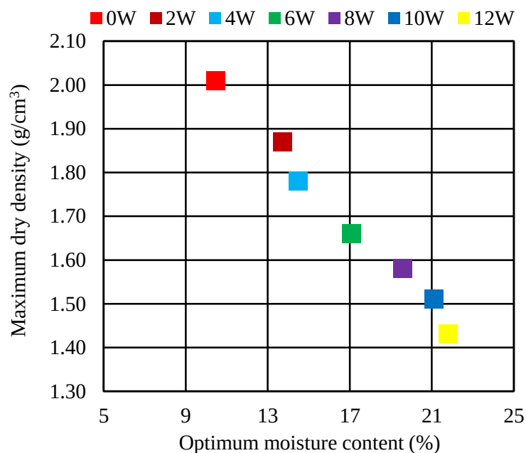
Fig. 3.17 Maximum dry density and optimum moisture content
