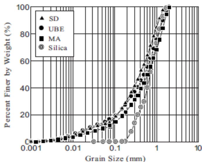
Fig. 2.7 Particle size distributions of decomposed granite soils (Ham et al. 2010)
