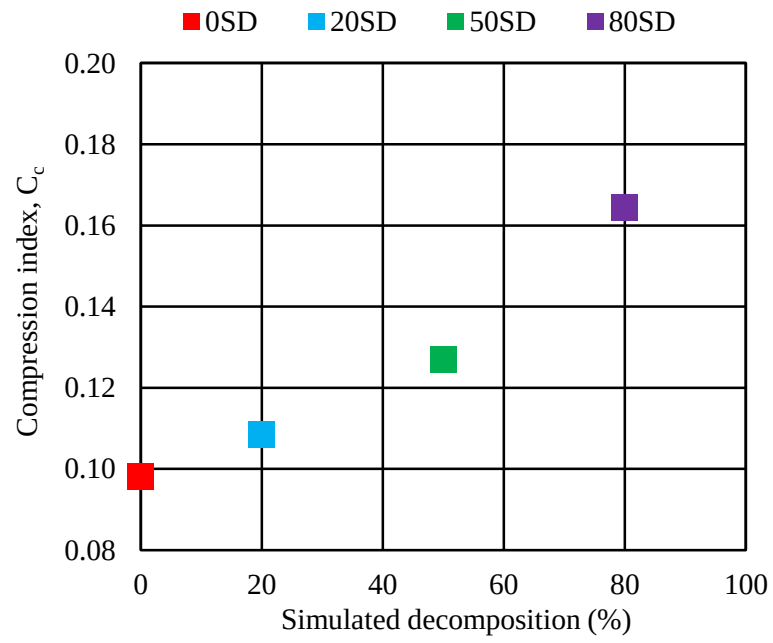
Fig. 4.14 Compression index versus simulated decomposition for basic sample 4W
