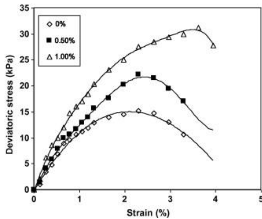
Fig. 2.8 Unconfined compression tests result at different percentages of plastic waste for sand (Babu and Choukesly 2011)
