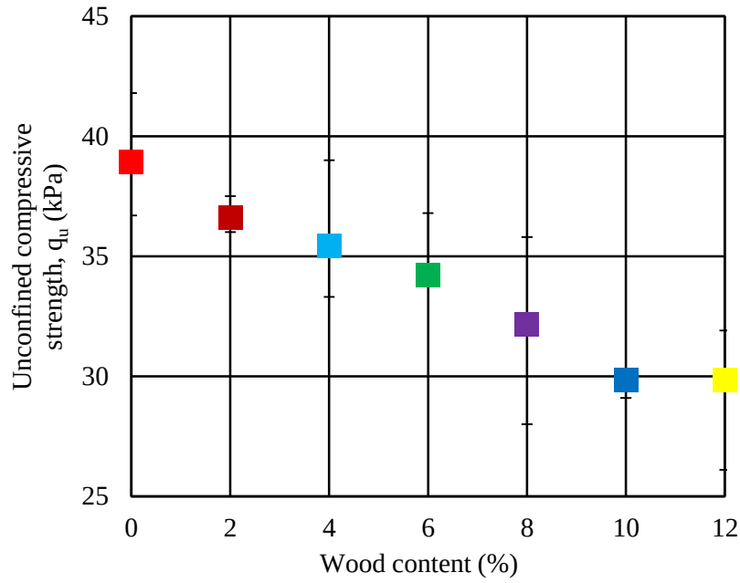
Fig. 3.19 Unconfined compressive strength and wood content
