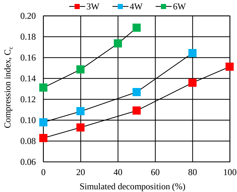
Fig. 4.16 Compression index versus simulated decomposition for all basic samples
