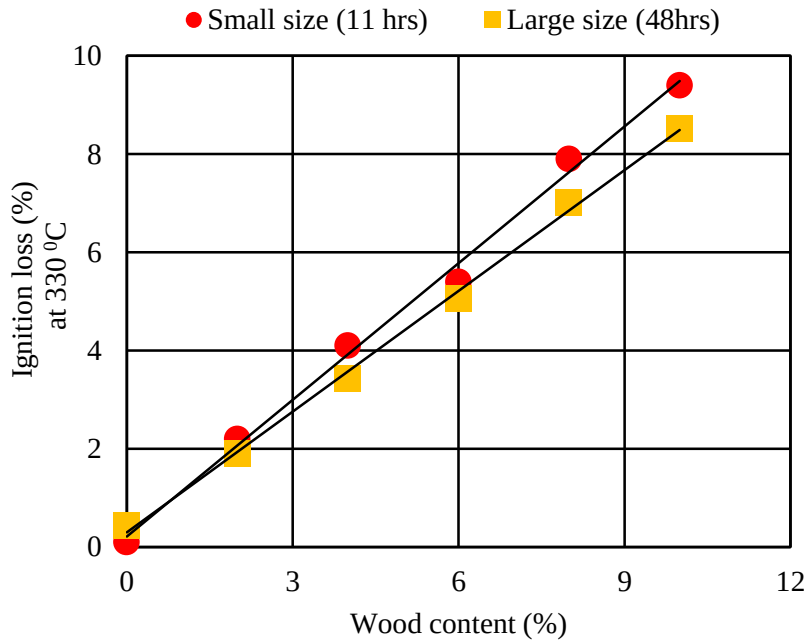
Fig. 3.7 Ignition loss and wood contents at different heating durations for both size
