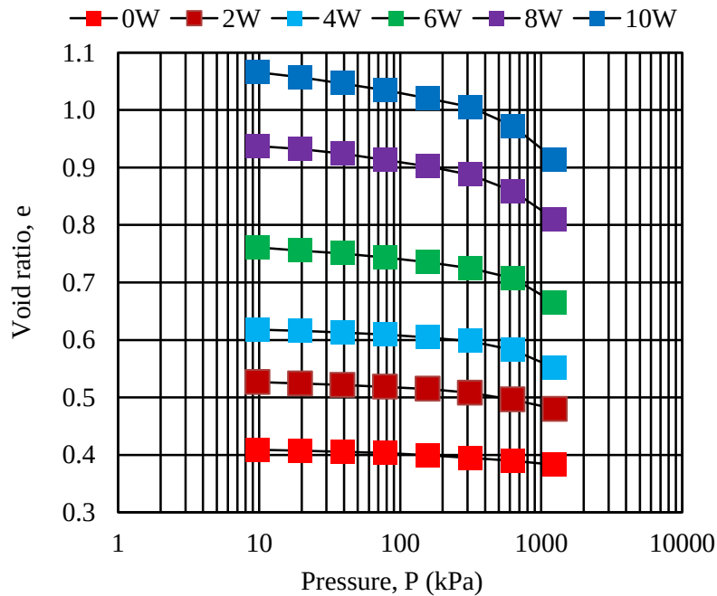
Fig. 3.25 Void ratio and pressure
