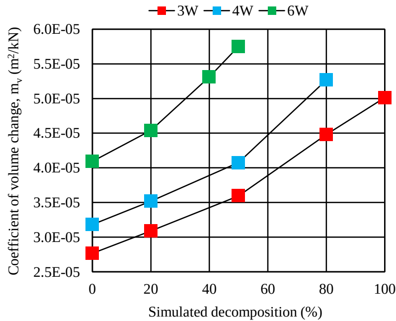
Fig. 4.29 Variation of volume changes with simulated decomposition for all basic samples
