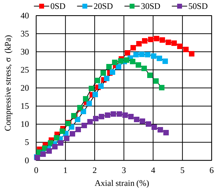
Fig. 4.3 Stress-strain relationship for various percentages of simulated decomposition for basic sample 6W
