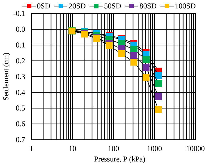
Fig. 4.21 Settlement versus pressure for basic sample 3W
