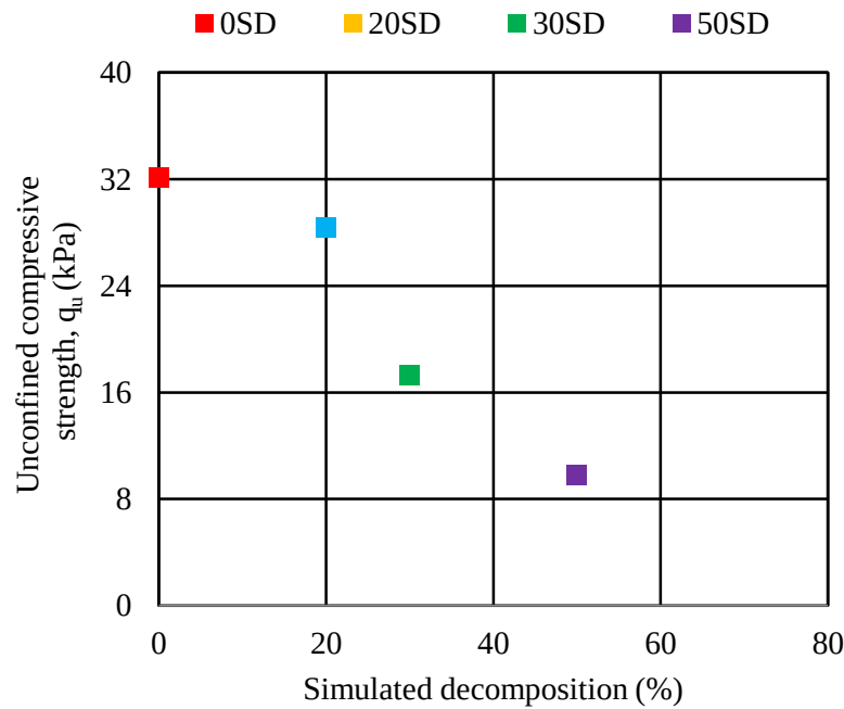
Fig. 4.7 Unconfined compression strength versus simulated decomposition for basic sample 8W
