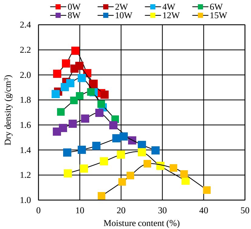
Fig. 3.12 Compaction curves of the samples with modified compaction test
