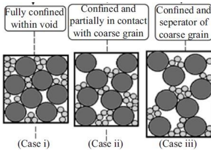
Fig. 3.34 Intergranular soil mix classification (Thevanayagam 2007)
