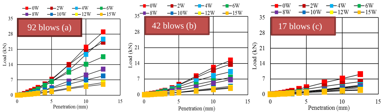
Fig. 3.21 load penetration curve at different blows
