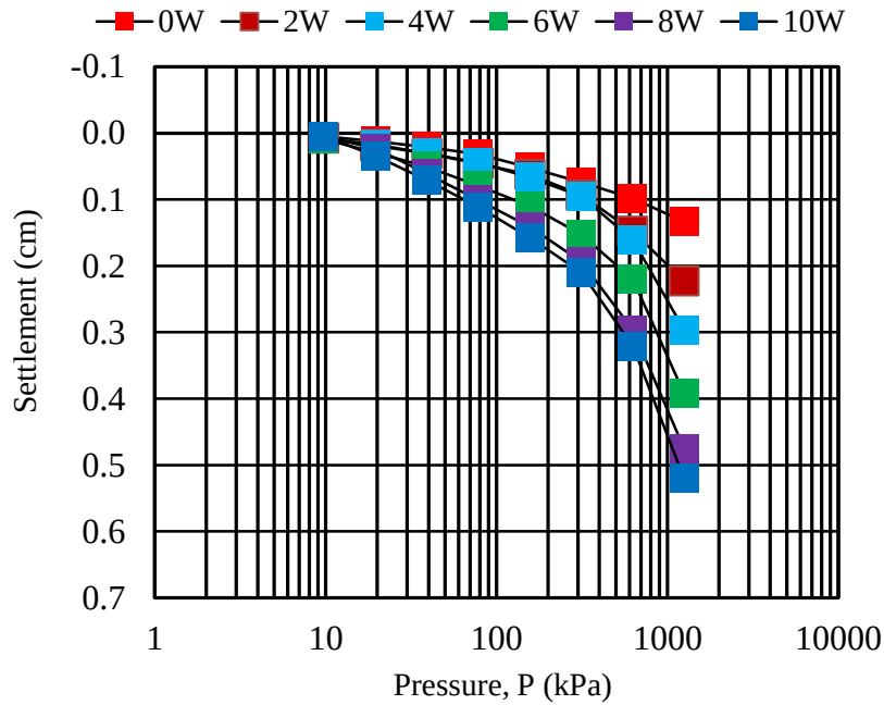
Fig.3.29 Settlement and pressure
