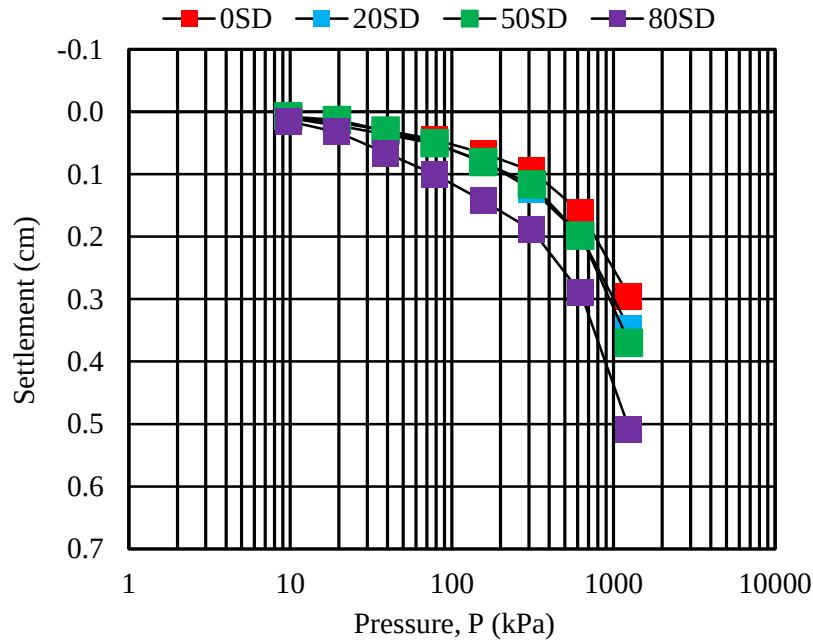
Fig.4.22 Settlement versus pressure for basic sample 4W
