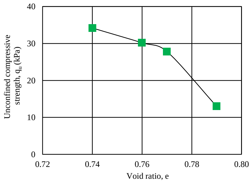
Fig. 4.26 Void ratio versus unconfined compressive strength for basic sample 6W
