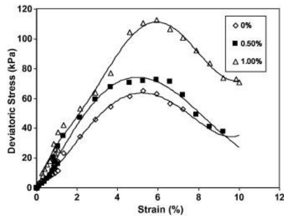
Fig. 2.9 Unconfined compression tests result at different percentages of plastic waste for red soil (Babu and Choukesly 2011)
