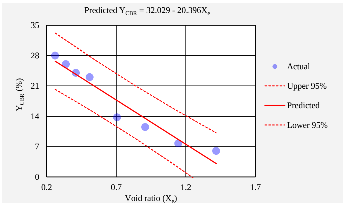
Fig. 3.38 Effects of void ratio on the predicted and observed CBR of recovered soil
