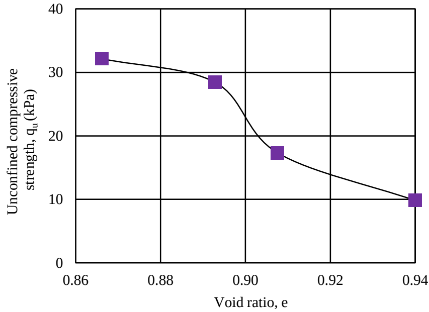
Fig. 4.27 Void ratio versus unconfined compressive strength for basic sample 8W
