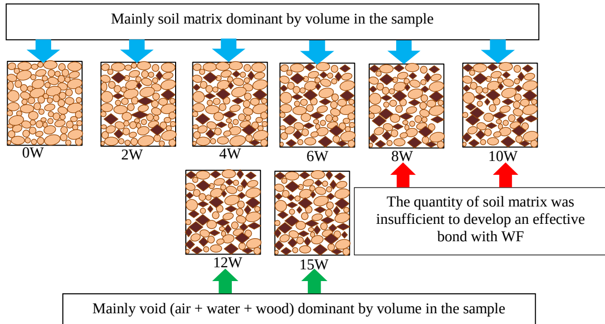
Fig.3.24 Conceptual diagram of wood-soil interactions at different samples
