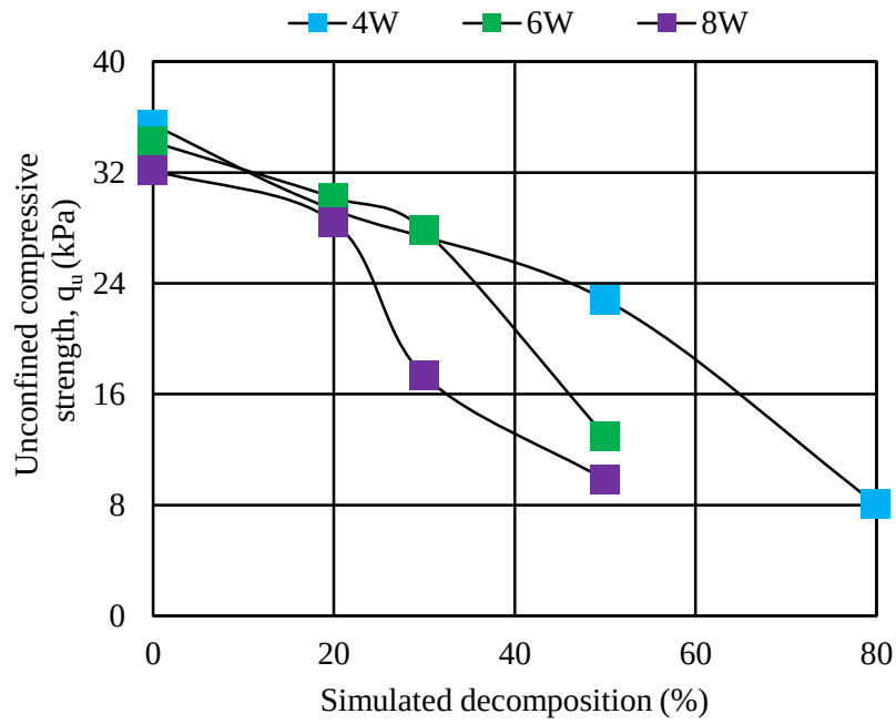
Fig. 4.8 Unconfined compression strength versus simulated decomposition for all basic samples
