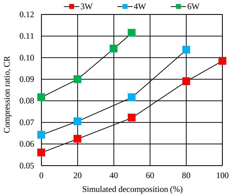
Fig. 4.20 Compression ratio versus simulated decomposition for all basic samples
