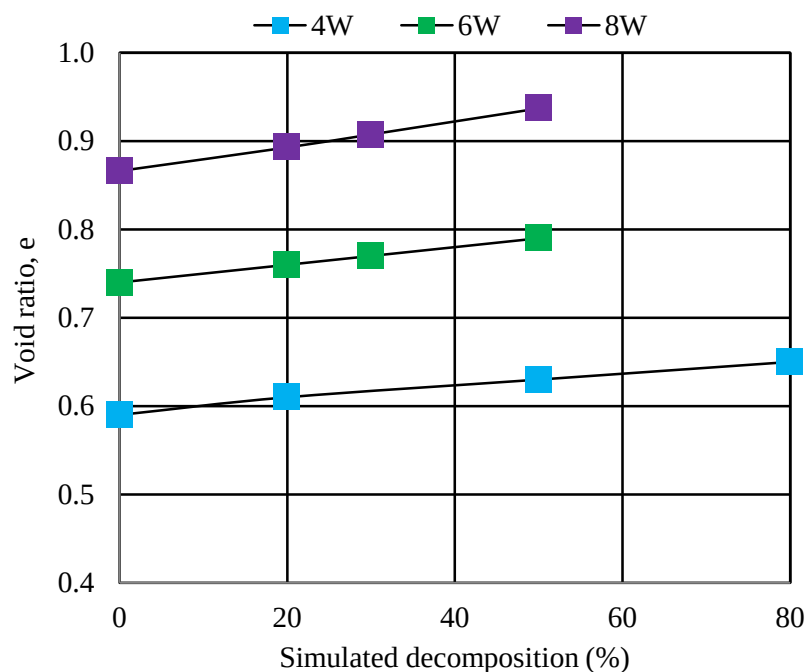
Fig. 4.24 Void ratio versus simulated decomposition for all basic samples
