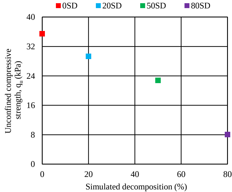
Fig. 4.5 Unconfined compression strength versus simulated decomposition for basic sample 4W
