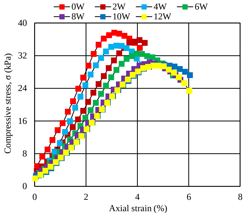
Fig. 3.18 Stress-strain relationship of the recovered soil
