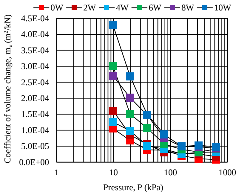
Fig. 3.37 Variation of volume changes versus pressure
