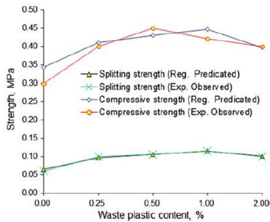
Fig. 2.10 Effects of plastic chips on the predicted and observed strength (Ahmed 2012)
