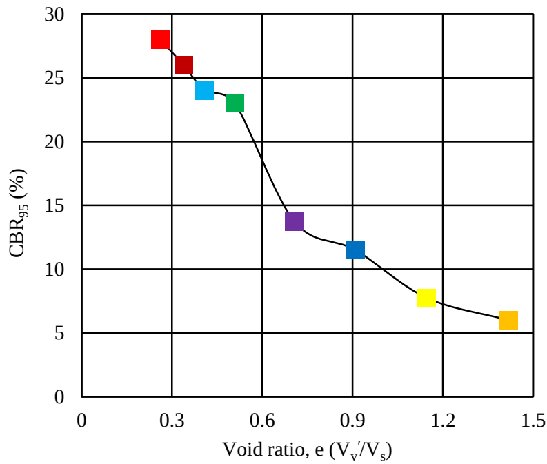
Fig. 3.35 CBR value versus void ratio ( V_v'/V_s )
