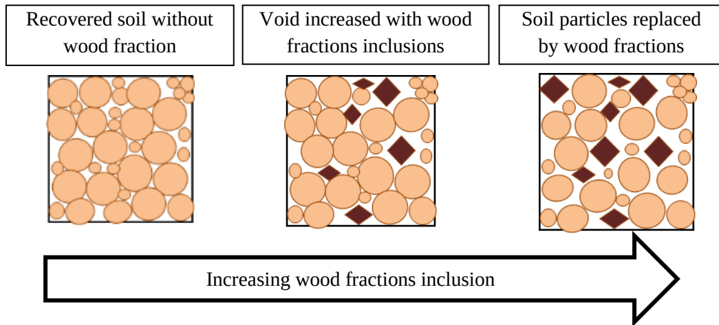
Fig. 3.33 Conceptual diagrams of soil particles and wood fractions interaction
