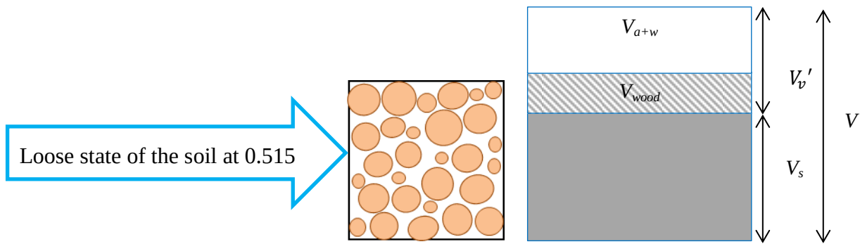
Fig. 3.39 Conceptual diagram of soil particles at loose state
