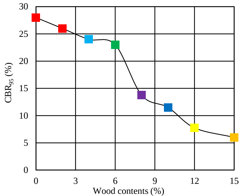
Fig 3.23 CBR value and wood contents
