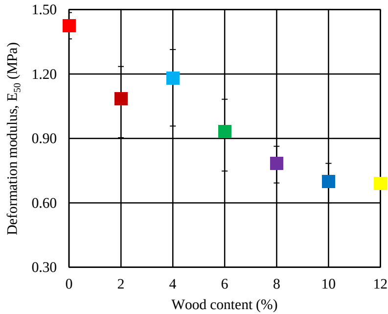
Fig. 3.20 Deformation modulus and wood content
