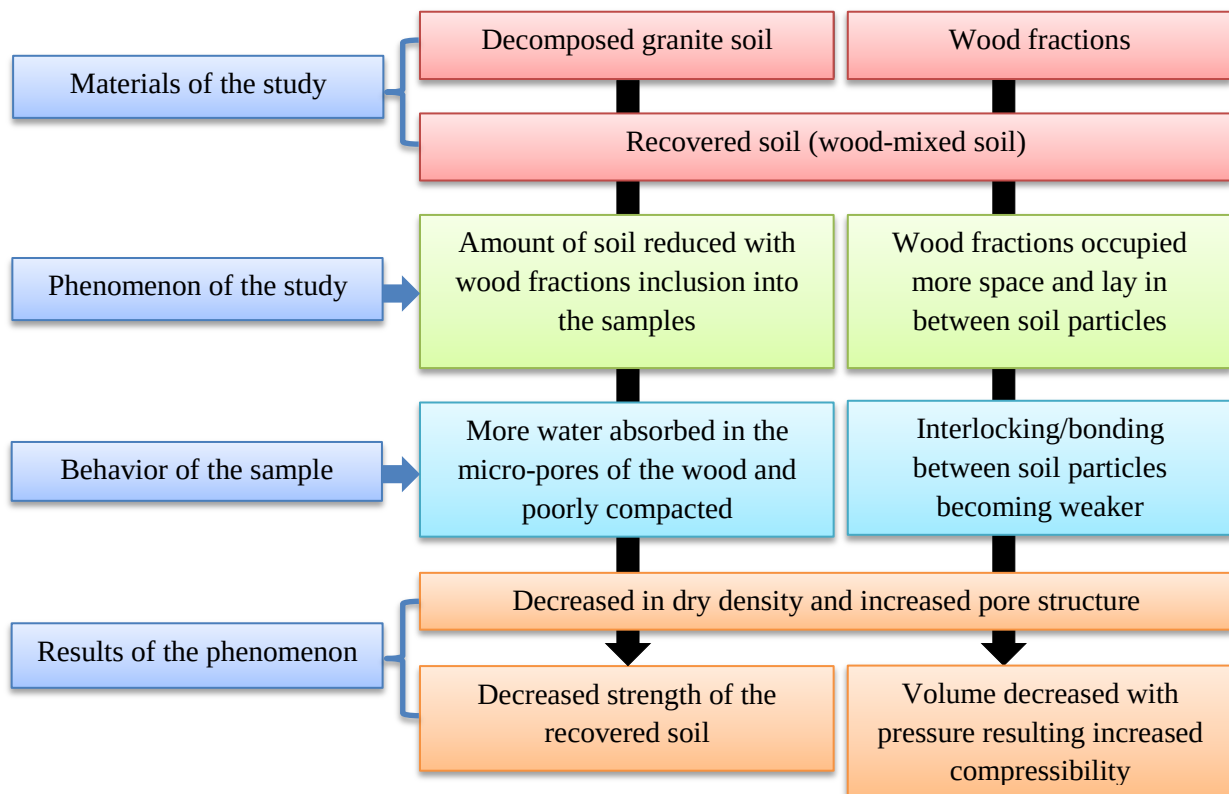
Fig. 3.42 Mechanism of soil-wood fractions interactions due to wood fractions inclusion
