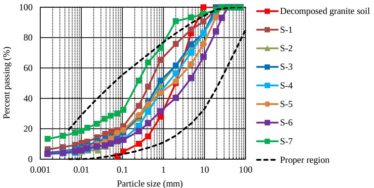
Fig. 3.2 Particle size distribution of affected sites soil along with decomposed granite soil
