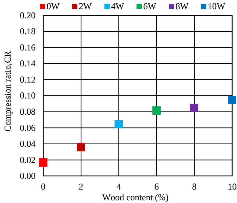
Fig. 3.28 Compression ratio and wood content
