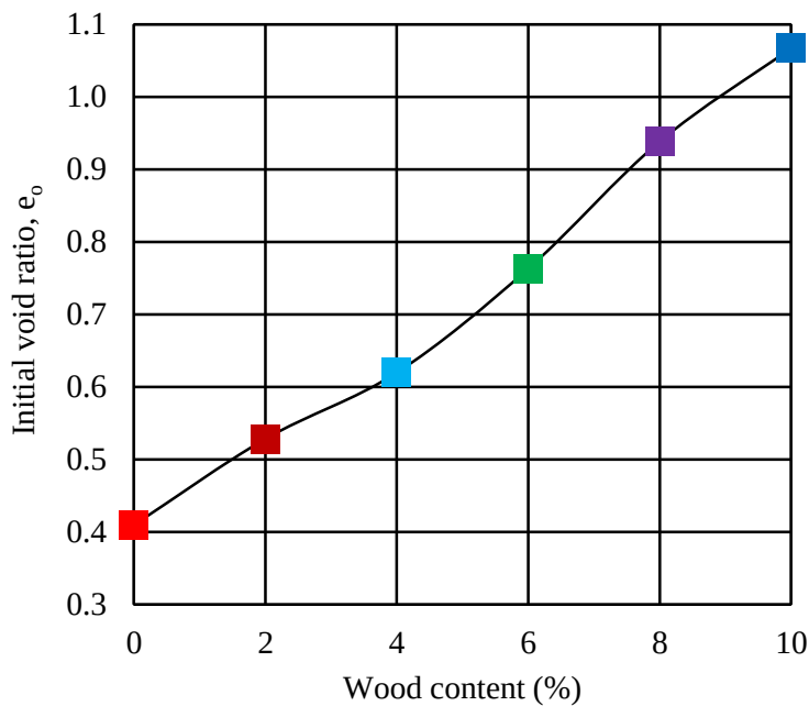
Fig. 3.26 Variation of initial void ratio with increase of wood fraction pressure
