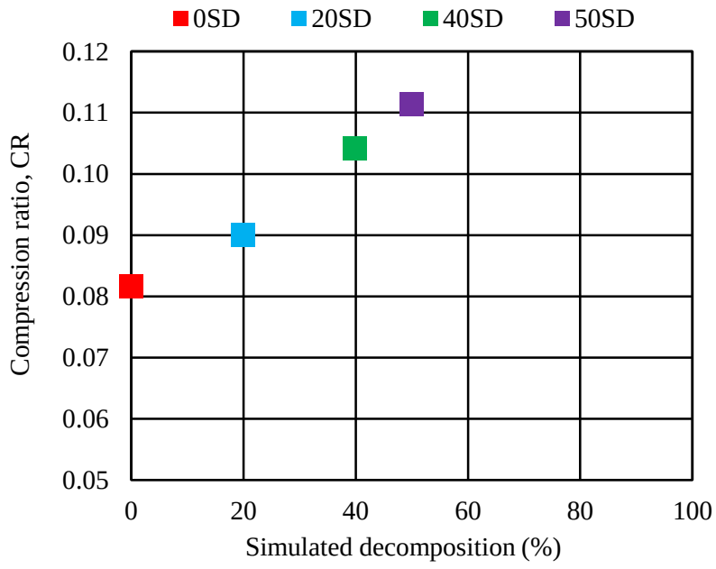
Fig. 4.19 Compression ratio versus simulated decomposition for basic sample 6W
