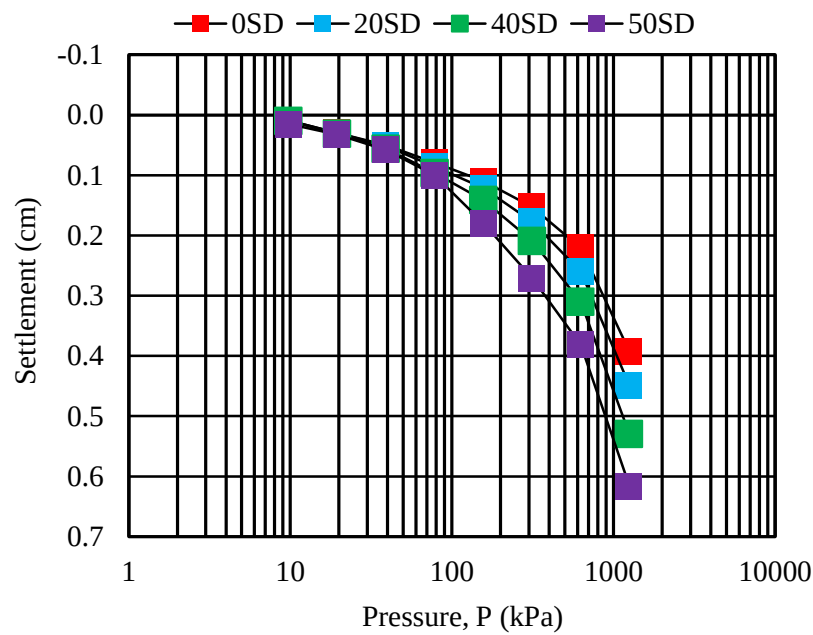
Fig. 4.23 Settlement versus pressure for basic sample 6W
