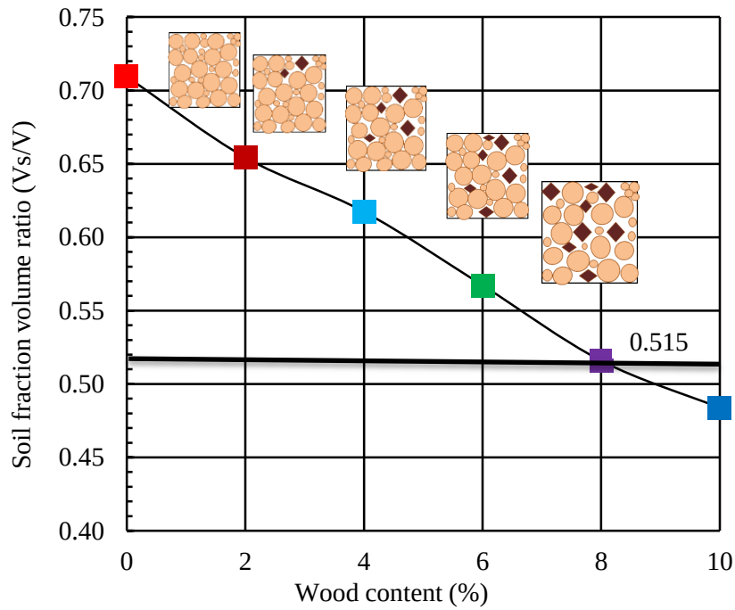
Fig. 3.41 Volume occupied with soil fraction relative to total volume of composite
