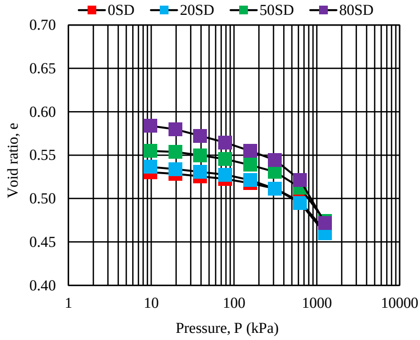
Fig 4.11 void ratio versus pressure for basic sample 4W
