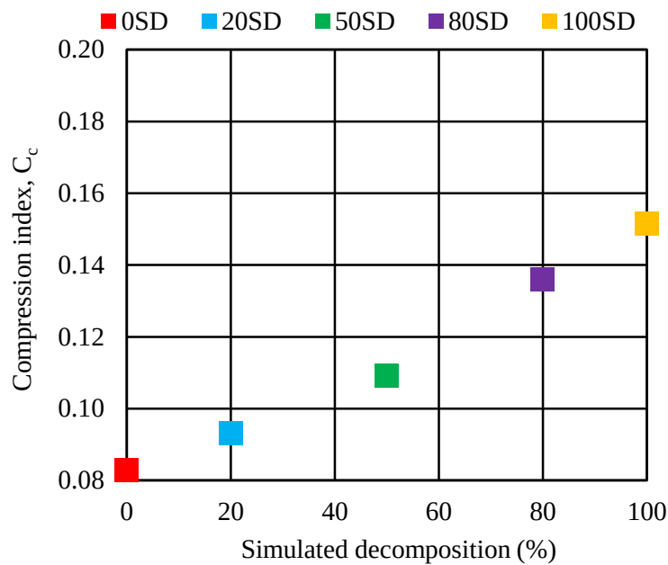
Fig. 4.13 Compression index versus simulated decomposition for basic sample 3W
