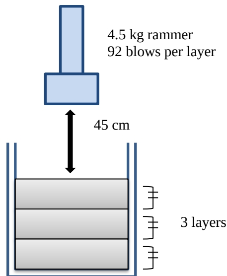
Fig 3.11 Schematic structure of the apparatus of compaction test along with specimen preparation
