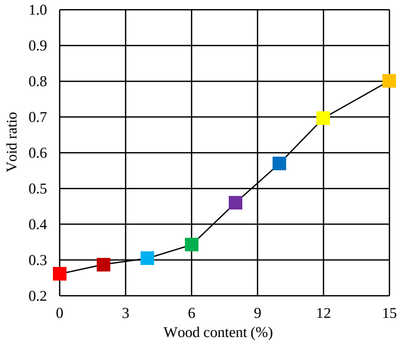
Fig. 3.31 Void ratio versus wood content
