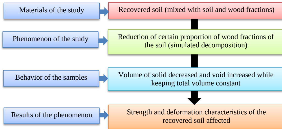
Fig. 4.30 Mechanism of soil-wood fractions interactions due to simulated decomposition
