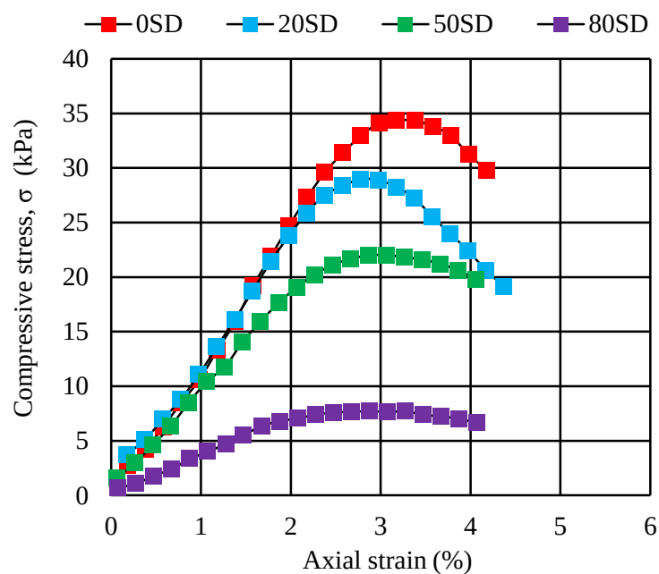
Fig. 4.2 Stress-strain relationship for various percentages of simulated decomposition for basic sample 4W
