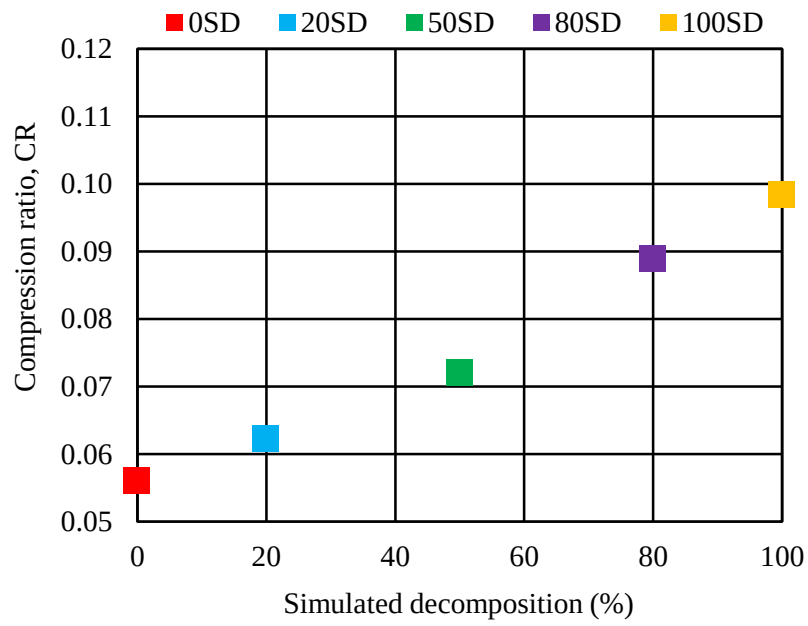
Fig. 4.17 Compression ratio versus simulated decomposition for basic sample 3W
