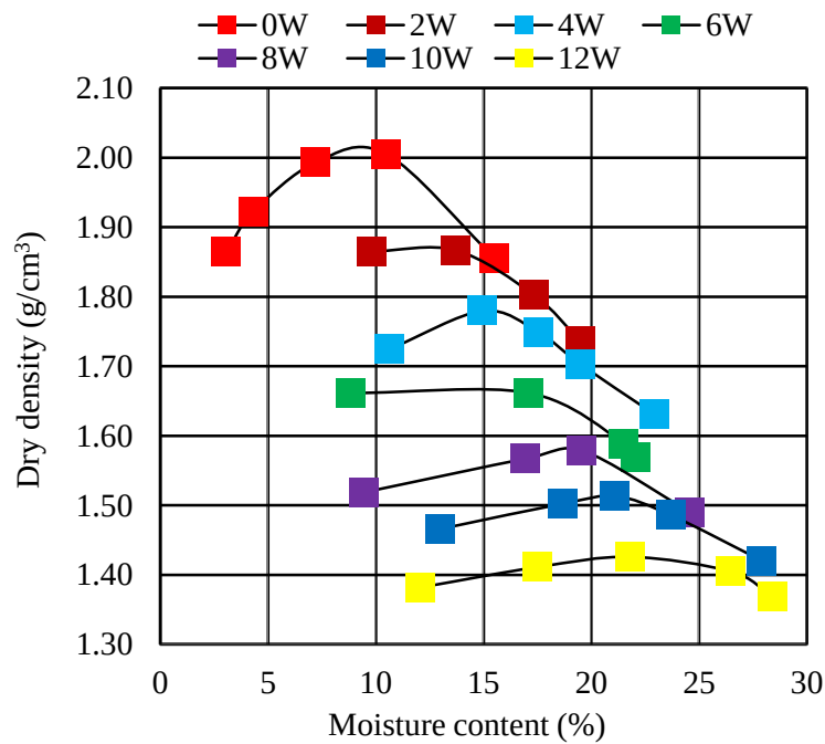
Fig. 3.16 Compaction curves
