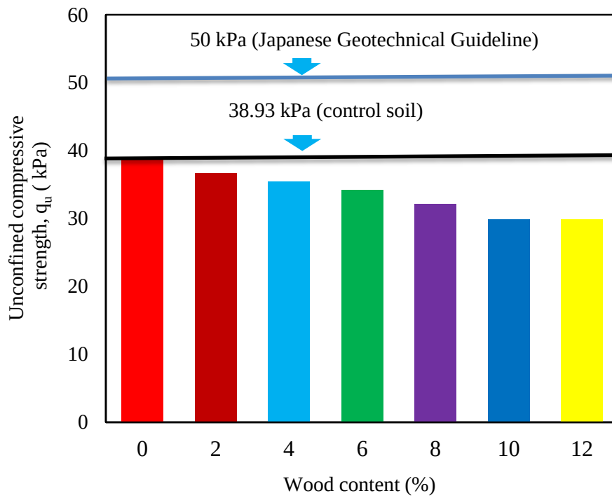
Fig. 5.1 Comparison of unconfined compressive strength of recovered soil with strength standard by JGG
