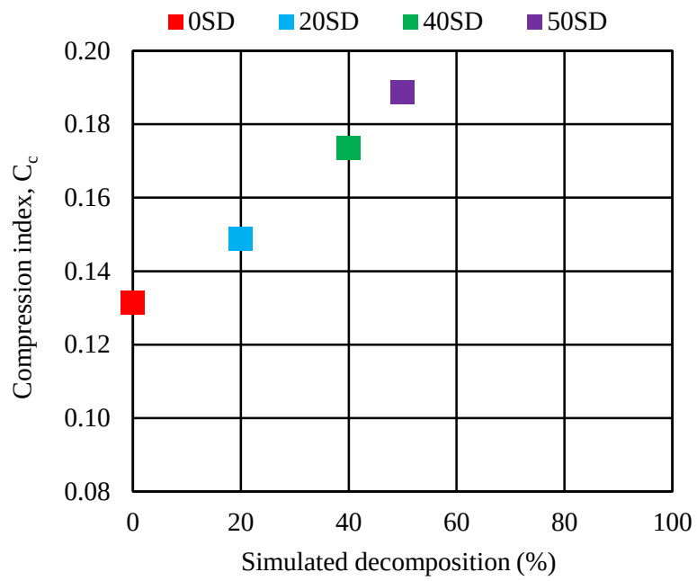
Fig. 4.15 Compression index versus simulated decomposition for basic sample 6W
