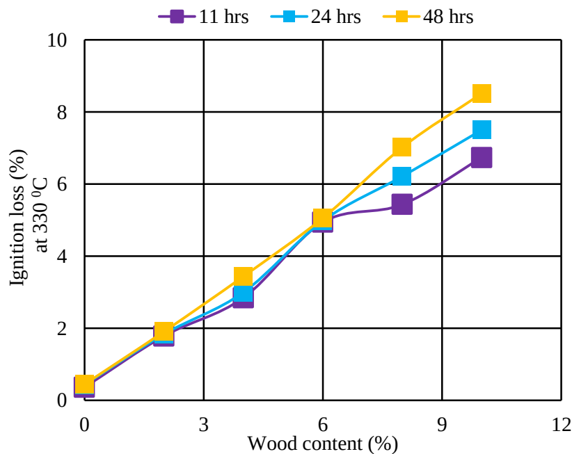
Fig. 3.6 Ignition loss and wood contents at three different heating durations with larger wood size
