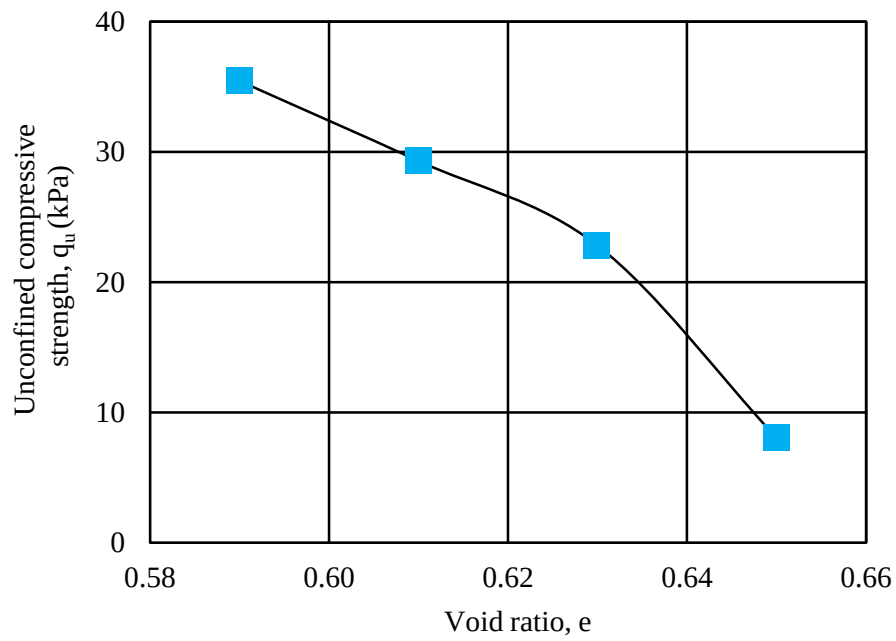
Fig. 4.25 Void ratio versus unconfined compressive strength for basic sample 4W
