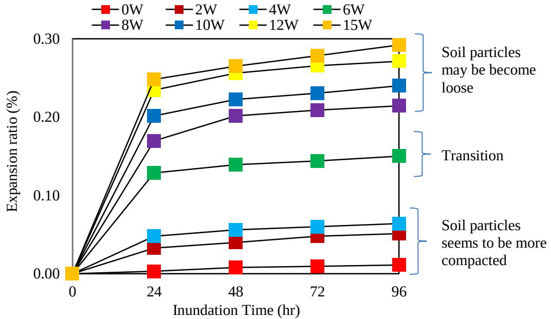
Fig. 3.22 Change of expansion ratio with time
