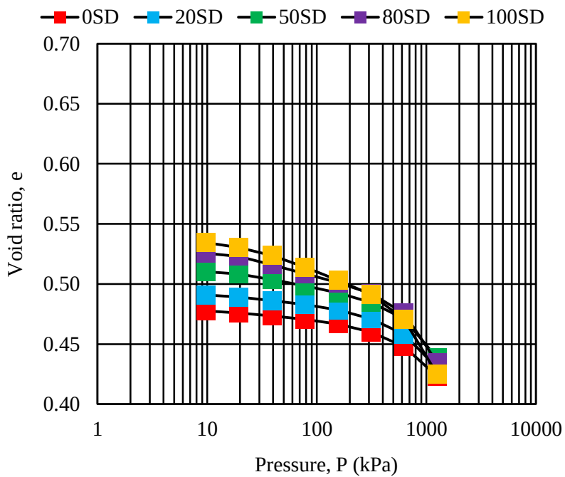
Fig. 4.10 void ratio versus pressure for basic sample 3W
