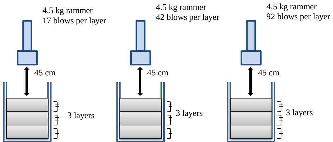
Fig. 3.13 Different compaction energy applied during specimens preparation
