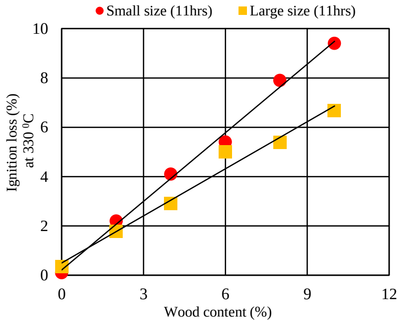
Fig. 3.8 Ignition loss and wood contents at same heating duration and temperature (11 hrs at 330°C)
