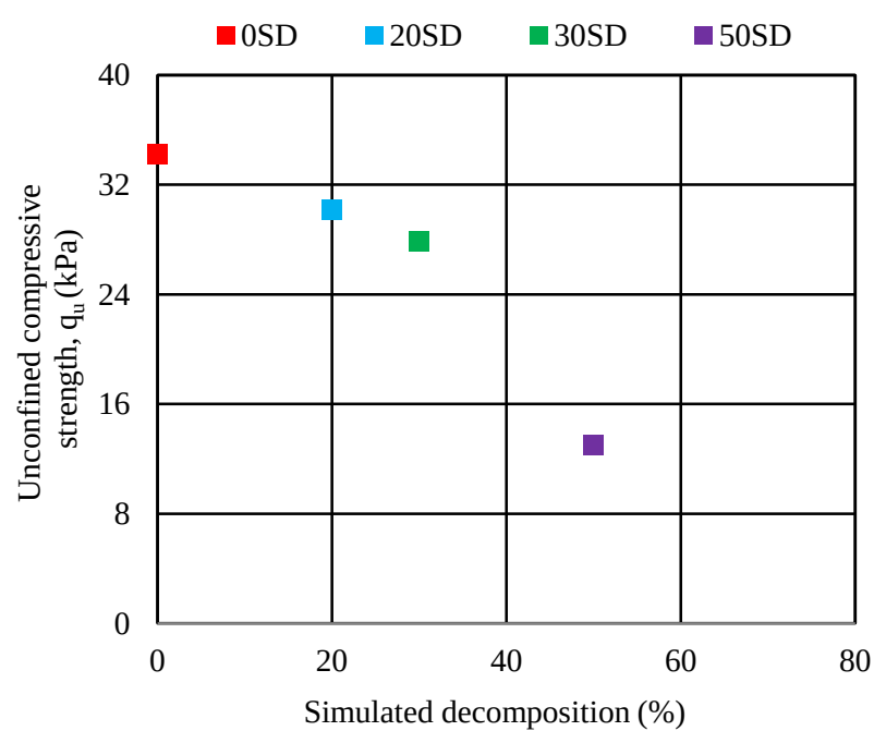
Fig. 4.6 Unconfined compression strength versus simulated decomposition for basic sample 6W
