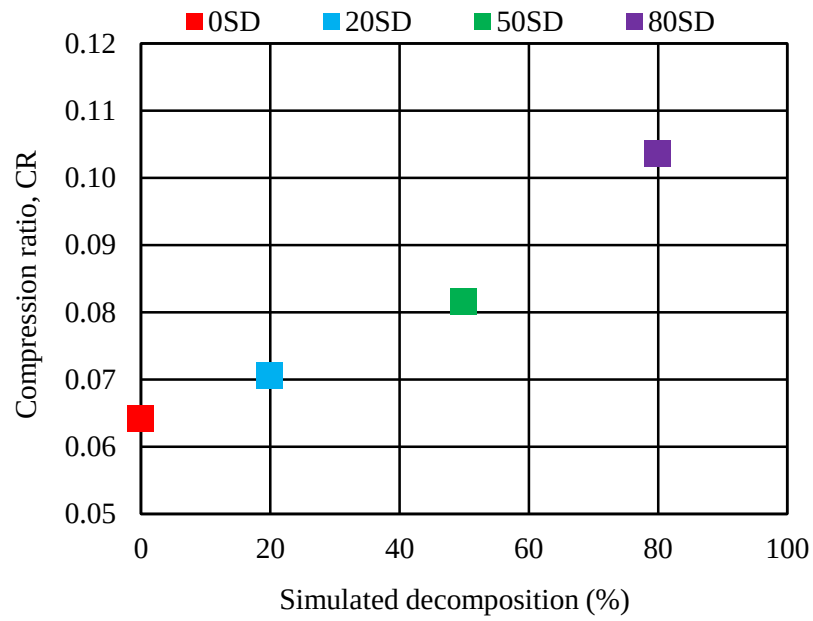
Fig. 4.18 Compression ratio versus simulated decomposition for basic sample 4W
