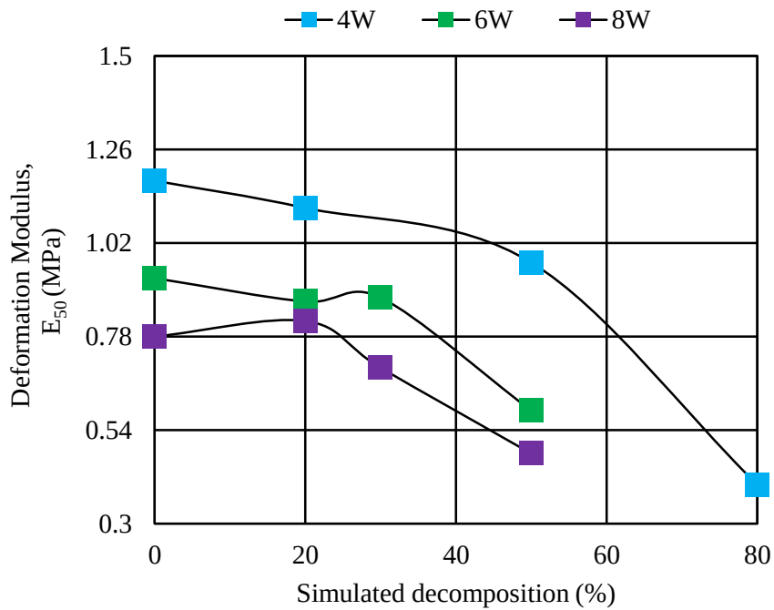
Fig. 4.9 Deformation modulus versus simulated decomposition for all basic samples
