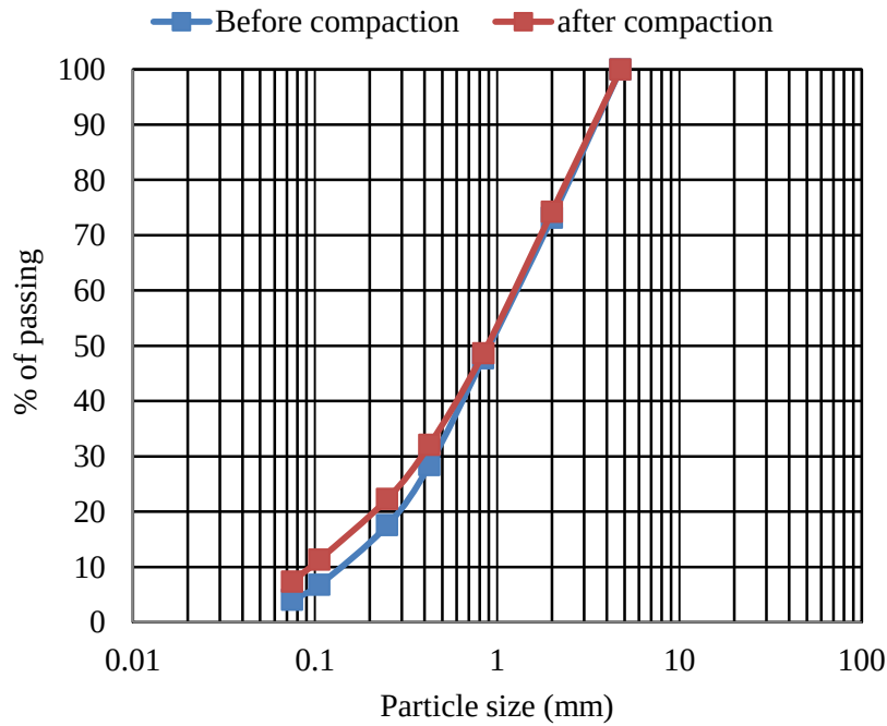
Fig. 3.32 Particle size distribution of recovered soil at after and before compaction
