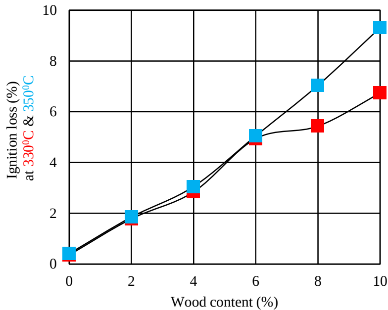
Fig 3.3 Ignition loss and wood contents
