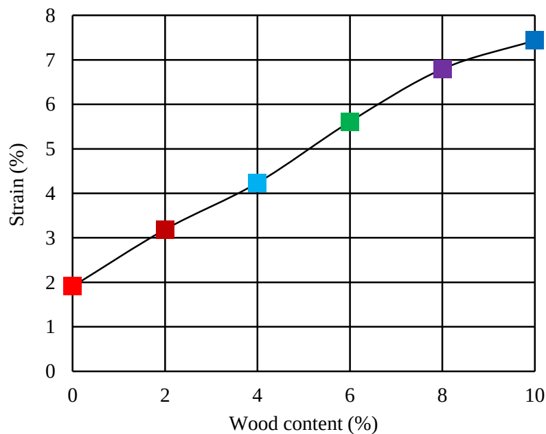
Fig. 3.30 Strain and wood content
