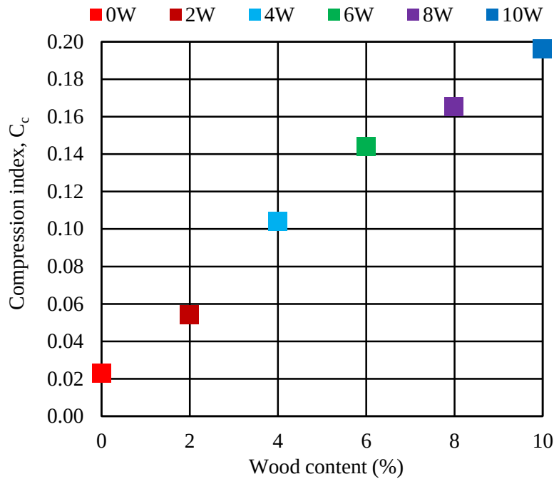
Fig. 3.27 Compression index and wood content
