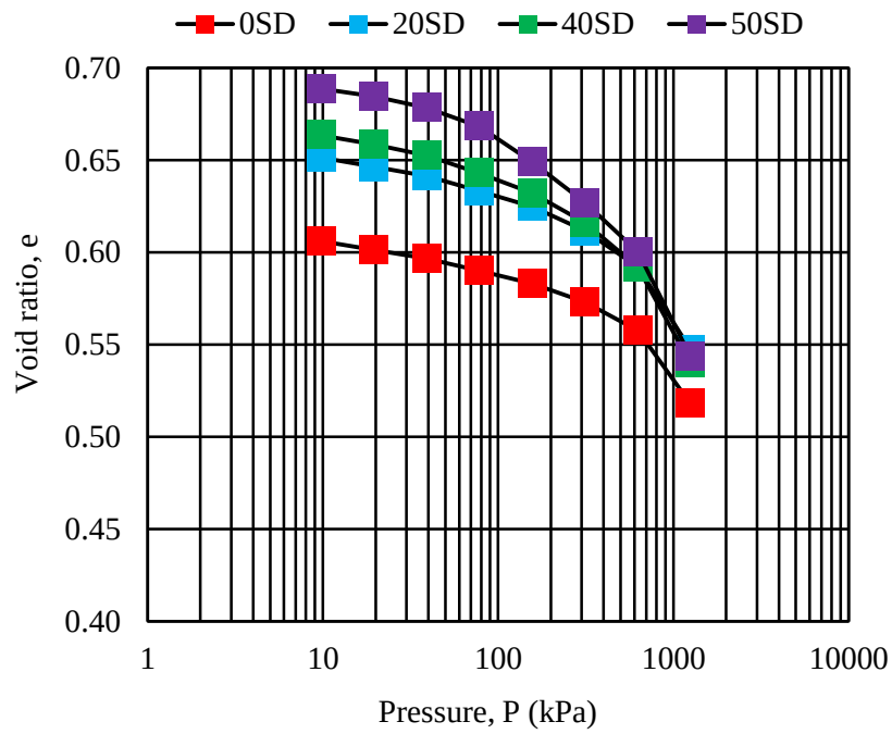
Fig. 4.12 void ratio versus pressure for basic sample 6W
