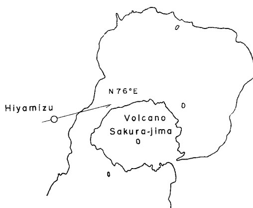
Fig. 4. Position of the Hiyamizu Station and the direction of the recording water tube tiltmeter.
