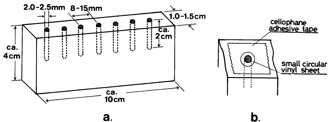
Fig. 1. Wood blocks with holes accommodating the larvae.
