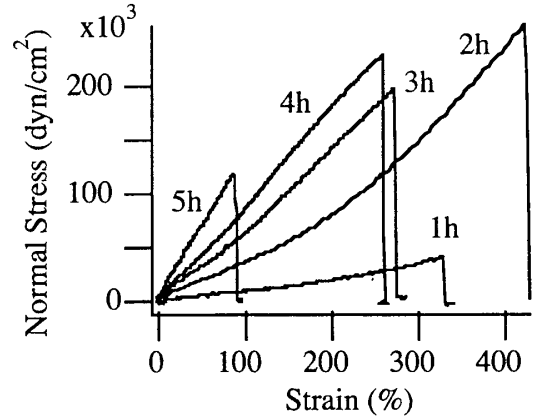
Figure 1: Stress-strain curve of topological gels in the gelation process.
