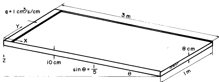
Fig. 1 Sketch of experimental slope.
