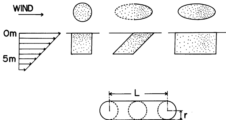
Fig. 8. Schematic representation of shear effect, namely the dispersion.
