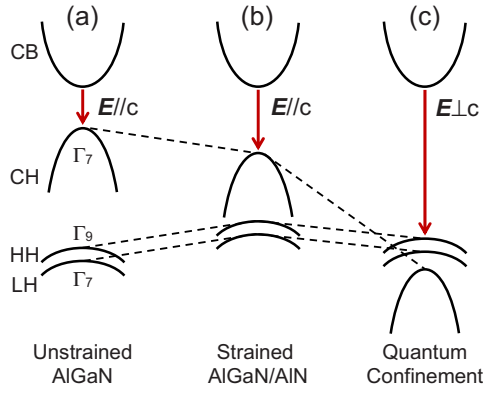
FIG. 4. (Color online) Schematic of band structures for (a) unstrained \text{Al}_x\text{Ga}_{1-x}\text{N} , (b) strained \text{Al}_x\text{Ga}_{1-x}\text{N} on unstrained AlN, and (c) \text{Al}_x\text{Ga}_{1-x}\text{N}/\text{AlN} QWs near the \Gamma point. CB and LH denote the conduction band and light hole band, respectively.
