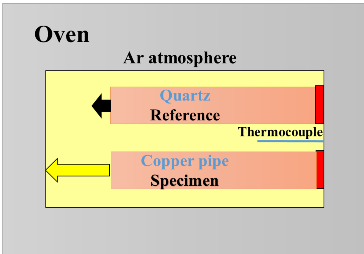
Figure 26. Schematic illustration of the thermal expansion meter.
