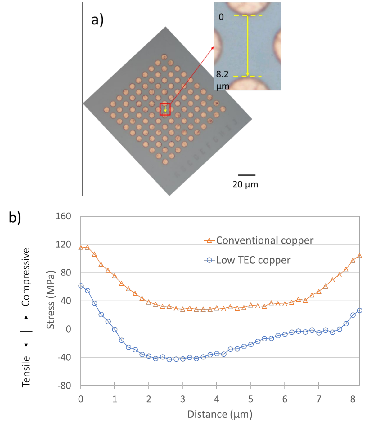
Figure 47. Stress measurement by micro-Raman spectroscopy
