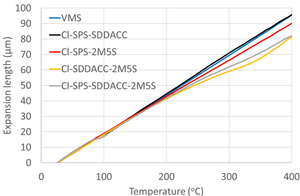
Figure 43. Thermal expansion of copper pipes electrodeposited with different additive combinations.
