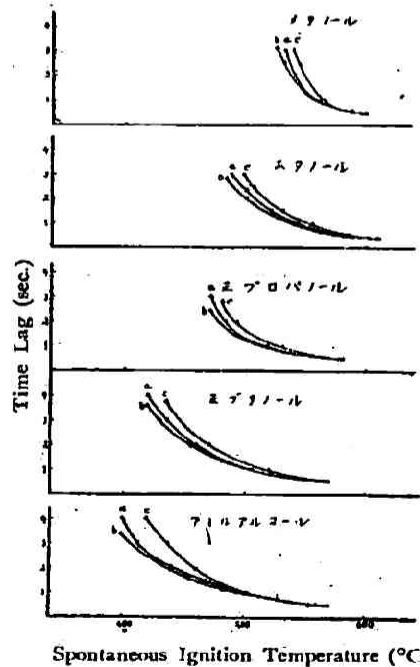
Fig. 5 F. Effect of antidetonants upon alcohols.
