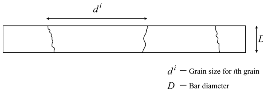
Figure 2. Typical bamboo-like grain structure for Cu-Al-Mn SEA bar with relatively large grain size.
