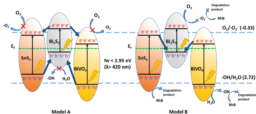
Figure 8. Proposed charge-transfer pathway models and RhB degradation mechanism of BiVO 4 /Bi 2 S 3 /SnS 2 under visible light illumination.
