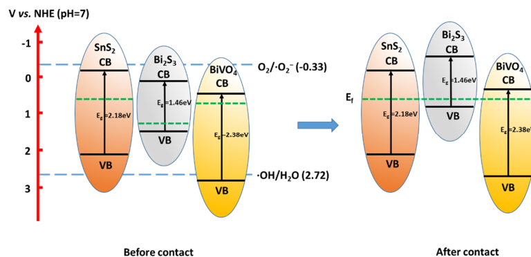
Figure 7. Band energy structures of BiVO 4 , Bi 2 S 3 , and SnS 2 before and after contact.
