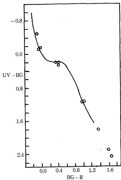
Fig. 9. Two-color diagram of Tifft's system. Symbols are the same as in Fig. 5. Plotted stars consist of the standards in and near NGC 6910 and NGC 6913 and Johnson-Morgan's.
