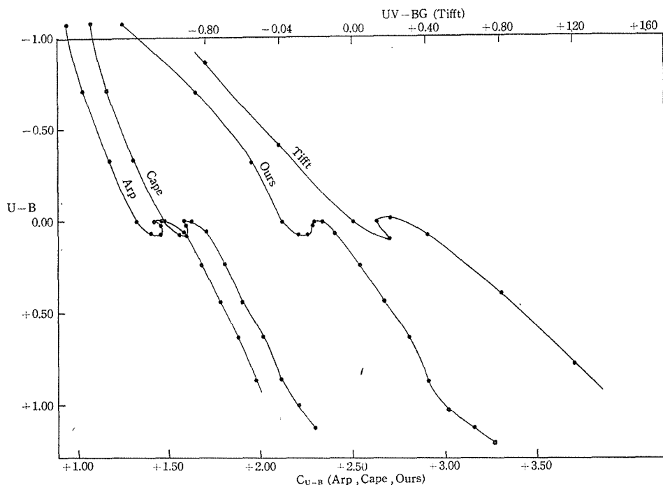
Fig. 12. Comparison of C_{U-B} 's of various systems against the standard U-B .
