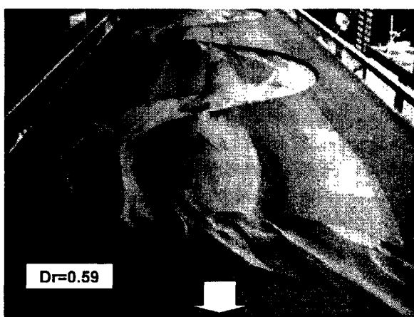
Photo.3 Bed form in the case of rough flood plain. ( Q=45.56 l/s, U_m=29.8 cm/s, h_f=5.69 cm)
