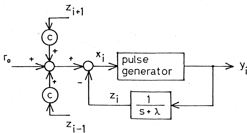
Fig.2 Neuron model.
