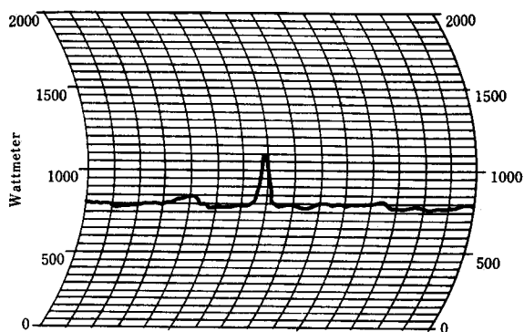
Figure-6. electric power consumption graph in the case that a brush cutter edge is caught in the stump.
