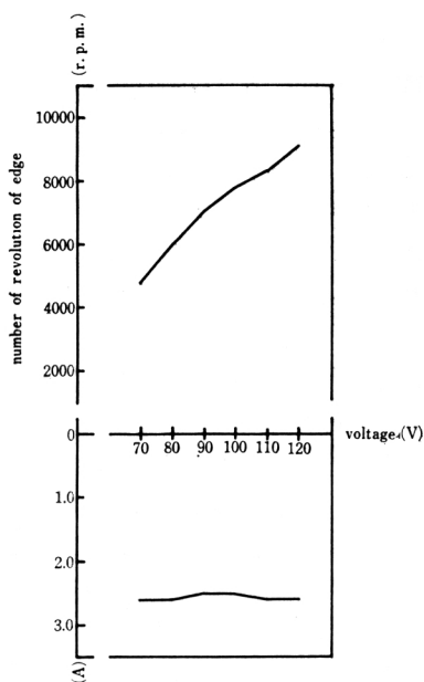
Figure-7-2. The relation between number of revolution of edge or amperage and voltage in the case of FC-2 type.
