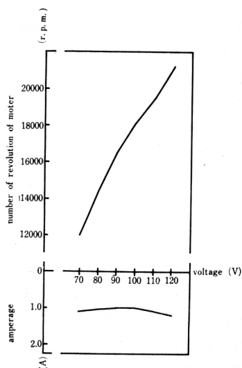
Figure-7-5. The relation between number of revolution of motor or amperage and voltage in the case of FC-4 type 85Y 5520.
