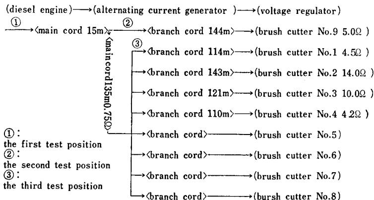
Figure-5. Illustration of the placement of brush cutters.
