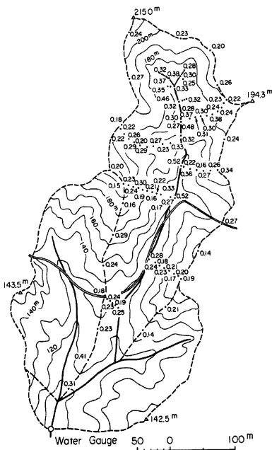
Fig. 3 Soil moisture contents measured on July 17, 1981.
