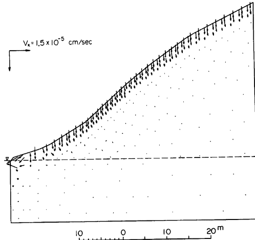
Fig. 15 Calculated velocity distribution on July 6, 1981.
