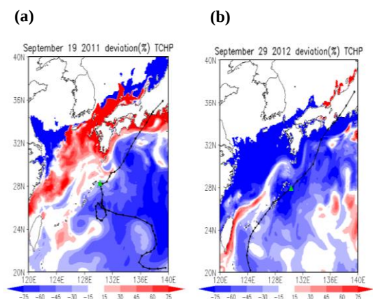
Fig.21 TCHP deviation in percentage.
