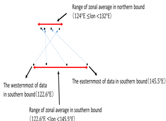
Fig.3 Illustration showing the zonal range of sea level pressure averaging. A blue dashed arrow connects TC location at southern and northern bounds of objective area. Zonal averaging is conducted between the westernmost and easternmost longitudes.
