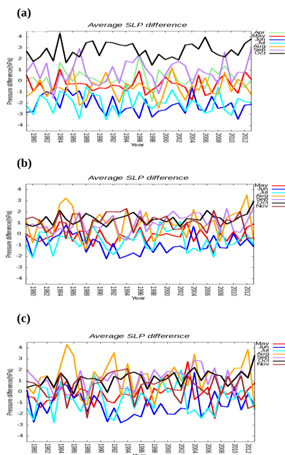
Fig.4 Sea level pressure difference between southern and northern bounds of April to November from 1979 to 2013.
