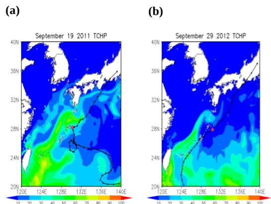
Fig.20 The TCHP distribution. Legends are the same as the former figures.
