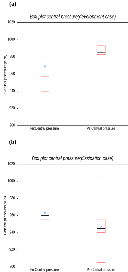
Fig.8 Box plot showing the distribution of p_s and p_n in summer season (July to September). The cross (X) corresponds to the average value, (a) \Delta p_c \leq -7.5\text{hPa} cases and (b) \Delta p_c > 7.5\text{hPa} cases.
