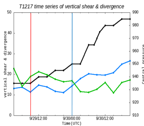
Fig.23 Time series of vertical shear (blue), horizontal divergence ( 10^{-6}\text{s}^{-1} ) (green) averaged within a circle of 500km radius from the TC center and central pressure (black) for T1115 (a) and T1217 (b). The red and blue lines are the same as Fig.11 and 13.
