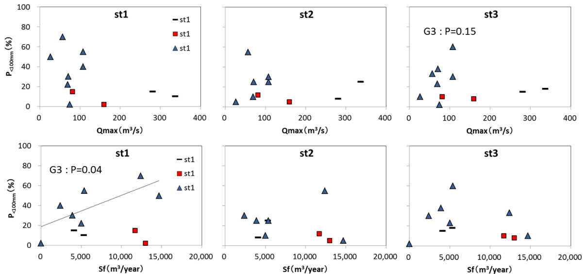
Fig. 5 Relationship between Q_{\max} , and P_{<100\text{mm}} (upper), and between S_f and P_{<100\text{mm}} (lower)
