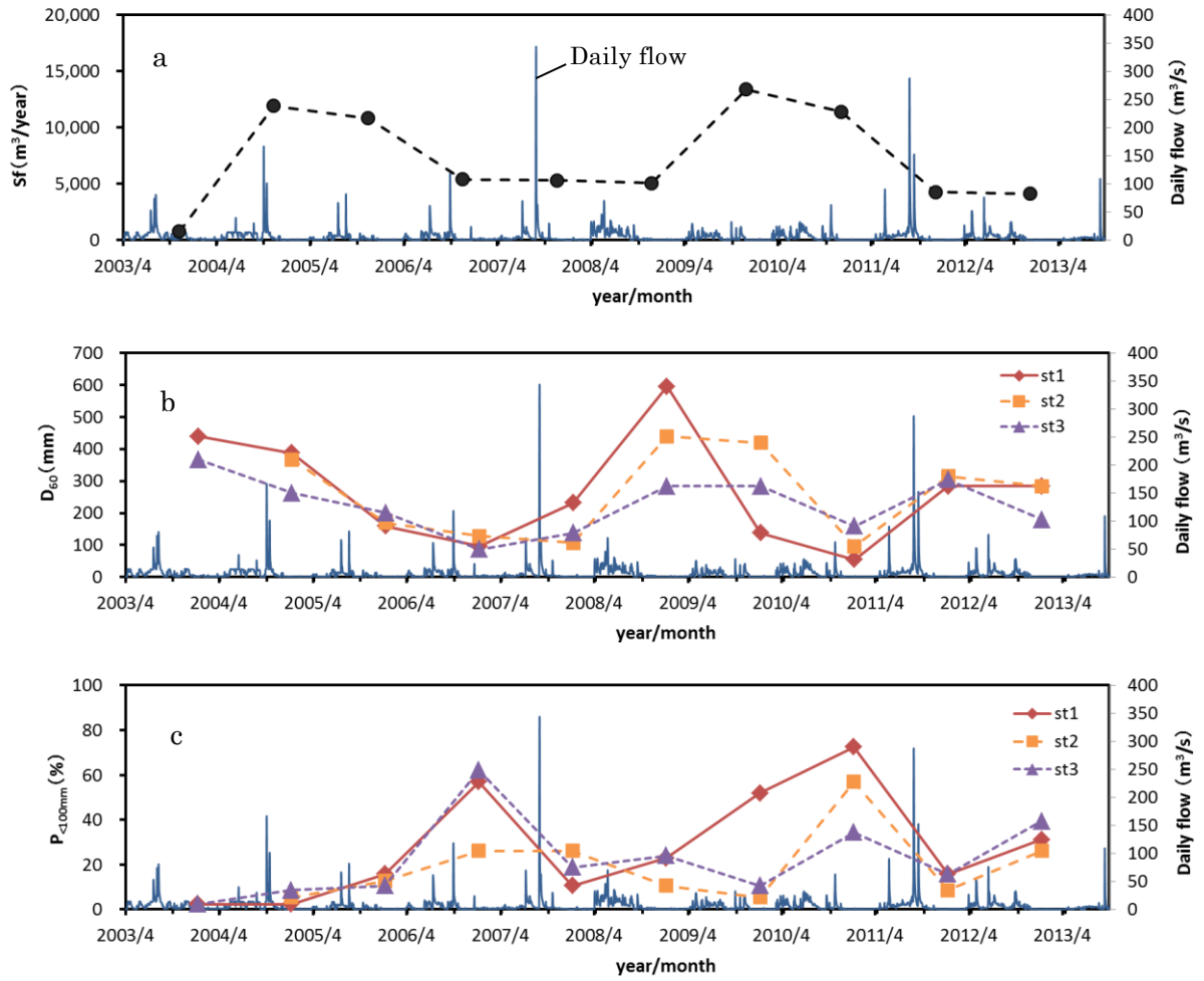
Fig. 3 The patterns of flow, Sf (a), D_{60} (b), and P_{<100mm} (c)
