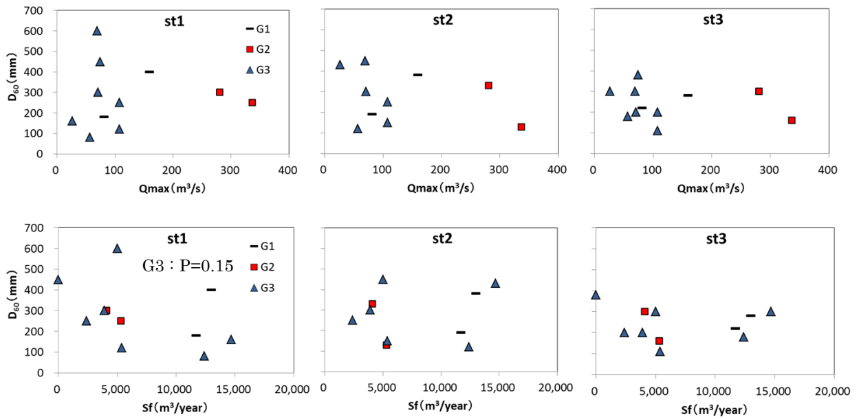
Fig. 4 Relationship between Q_{max} , and D_{60} (upper), and between Sf and D_{60} (lower)
