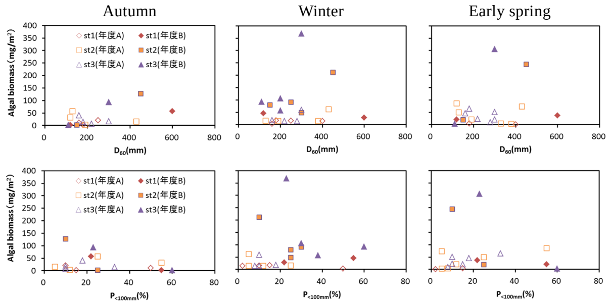
Fig. 8 Relationship between D_{60} and algal biomass (upper), and between P_{<100\text{mm}} and algal biomass (lower)
