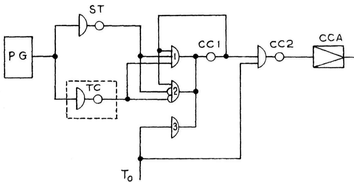
Fig.8.4-Coincidence circuit (CC).
