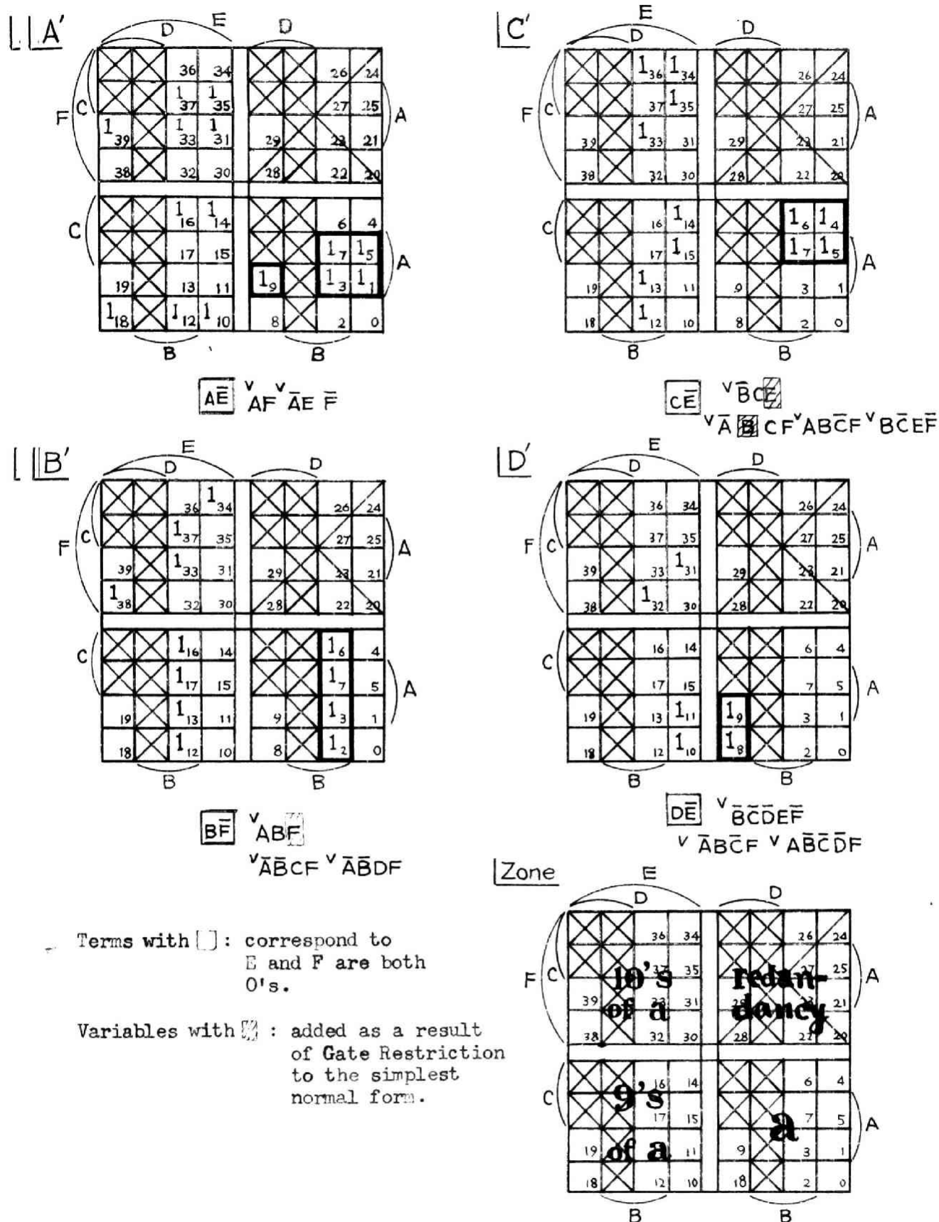
Fig.6.5 (2) - 10's Complementer; Veitch diagrams to obtain both the simplest normal forms and the simplest normal forms with the gate restriction.
