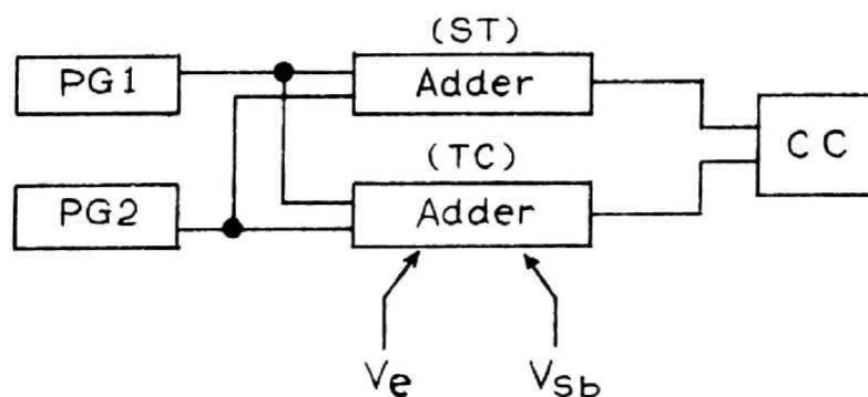
Fig.8.8-Measurement of the performance margin of an adder.
