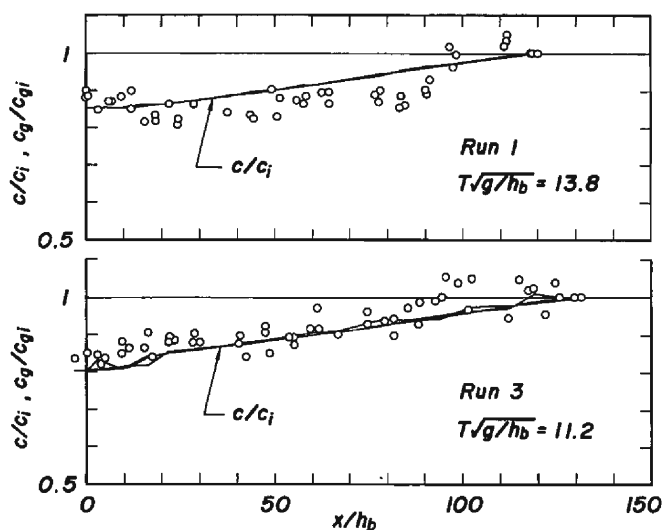
Fig. 15 Changes in group velocity over the slope based on the stream function theory.
