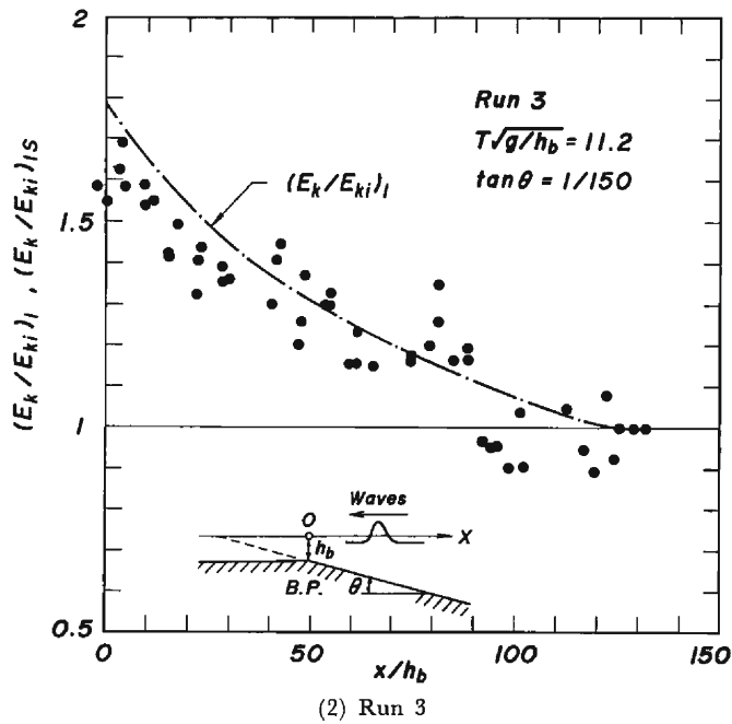
Fig. 16 Changes in kinetic energy over the slope based on the stream function theory.
