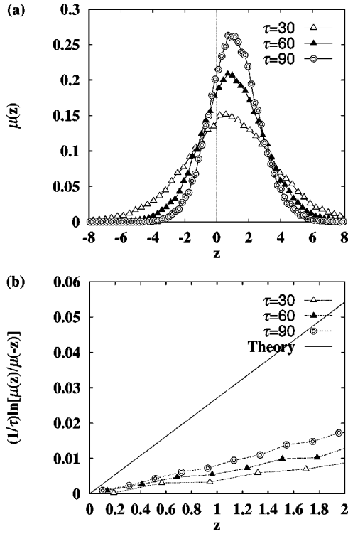
FIG. 9. Check of the ES identity. (a) Heat current distribution \mu_\tau(z) ( \tau=30,60,90 ) obtained from 50 000 random initial conditions. (b) J vs (1/\tau)\ln[\mu_\tau(z)/\mu_\tau(-z)] , \tau=30,60,90 . N=100, T_L=2.0, T_R=1.5 . The line labeled “Theory” corresponds to the theoretical slope \Sigma .
