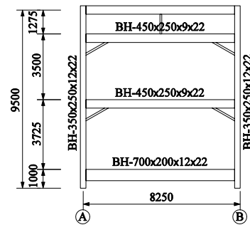
(c) Elevation of exterior N-S frame
