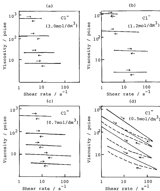
Fig. 8. Plots of viscosity versus shear rate for sol 4(a), sol 5(b), sol 6(c) and sol 7(d). Arrows show the direction of the change of shear rate.
