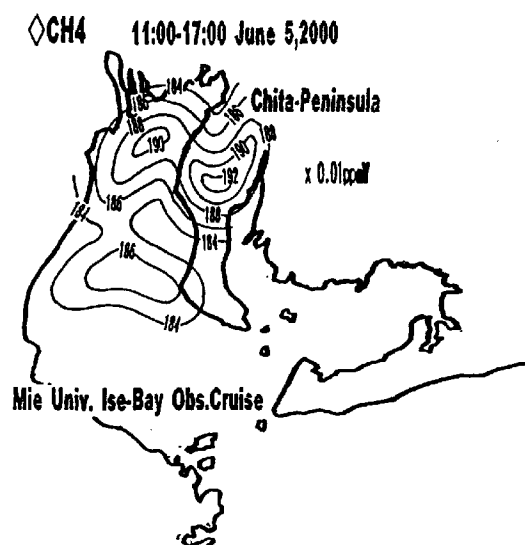
Fig.1 Spatial distribution of atmospheric methane concentration over Ise Bay and Chita-Peninsula during the time 11:00-17:00 June 5, 2000.
