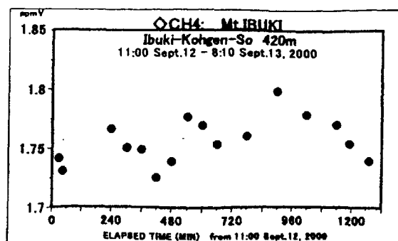
Fig. 5 Temporal variation of atmospheric methane concentration at Ibuki-Kohgen-So (420m) near Ibukiyama-Ski-Run.
