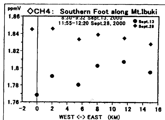
Fig. 6 Distribution of atmospheric methane concentration along the southern foot of Mt. Ibuki: Abscissa denotes the relative distance eastward.
