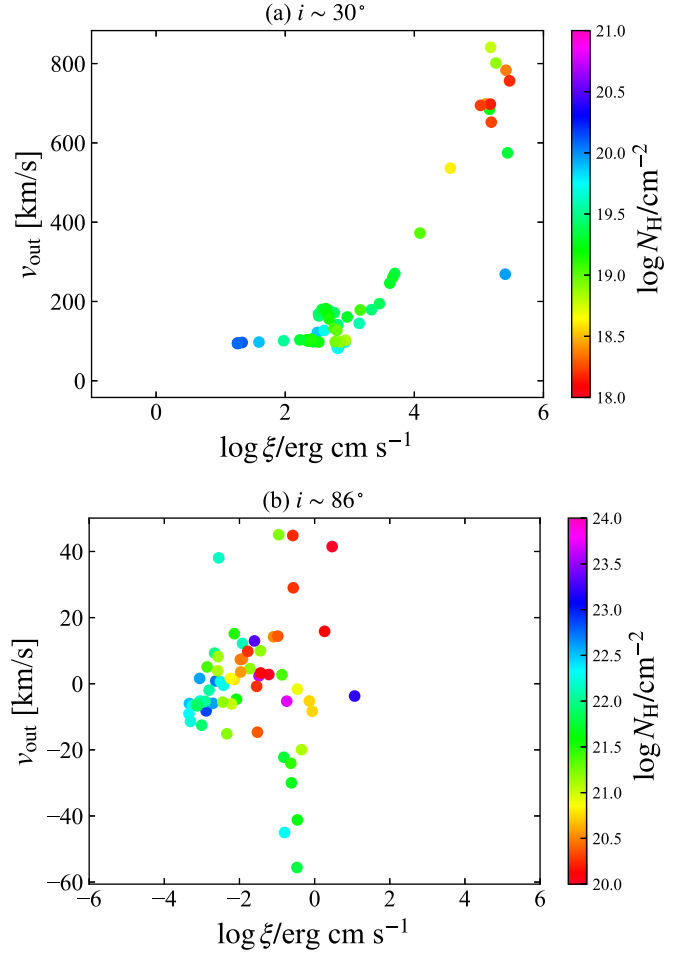
Figure 5. Relation between the ionization parameter ( \xi ) and outflow velocity ( v_{\text{out}} ) for the grid cells along a line of sight. Each data point is color-coded by the hydrogen column density in the cell. (a) For i = 30^\circ . (b) For i = 86^\circ .
