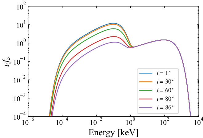
Figure 8. Incident SED models of NGC 4051 at the innermost grids for inclination angle of i = 1^\circ, 30^\circ, 60^\circ, 80^\circ , and 86^\circ (top to bottom). The vertical axis has an arbitrary unit of \nu f_\nu .
