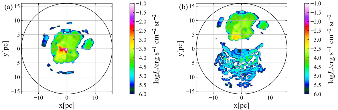
Figure 7. (a) Surface brightness distribution of O VIII Ly \alpha at 0.654 keV for the inclination angle i = 0^\circ . (b) Same as panel (a) but for i = 30^\circ .
