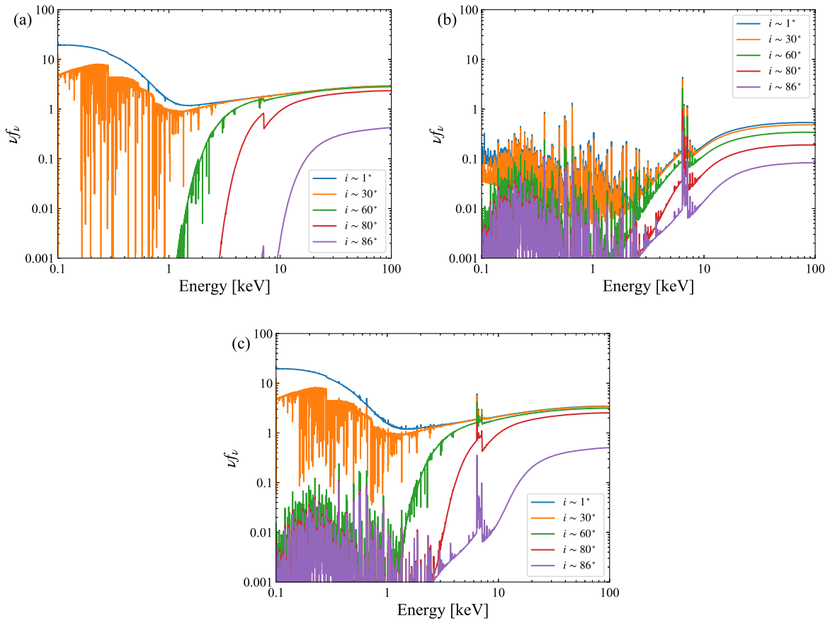
Figure 9. Simulated X-ray spectral models for NGC 4051 in units of \nu f_\nu for inclinations of i = 1^\circ , 30^\circ , 60^\circ , 80^\circ , and 86^\circ (top to bottom). (a) Transmitted spectra (attenuated incident radiation). (b) Scattered spectra, which contain Compton-scattered incident radiation and diffuse emission from all cells. (c) Total (transmitted + scattered) spectra.
