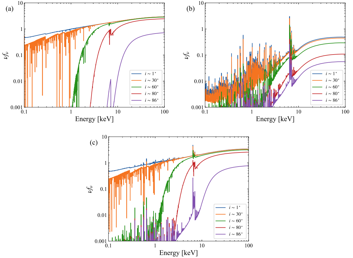
Figure 6. Simulated X-ray spectral models in units of \nu f_\nu for inclinations of i = 1^\circ , 30^\circ , 60^\circ , 80^\circ , and 86^\circ (top to bottom). (a) Transmitted spectra (attenuated incident radiation). (b) Scattered spectra, which contain Compton-scattered incident radiation and diffuse emission from all cells. (c) Total (transmitted + scattered) spectra.
