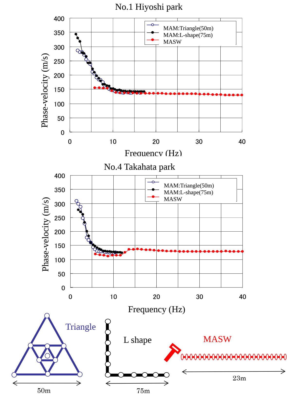
Figure 4.3.1 Comparison of passive and active dispersion curves in Nagoya, Japan.
