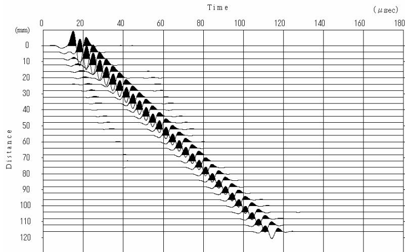
Figure 3.4.6. Synthetic waveform calculated by 3D elastic finite-different method. V_p=2500\text{m/s} , V_s=1300\text{m/s} , density= 1500\text{kg/m}^3 , grid spacing= 0.5\text{m} . P-wave source with 100\text{KHz} Ricker-wavelet is used.
