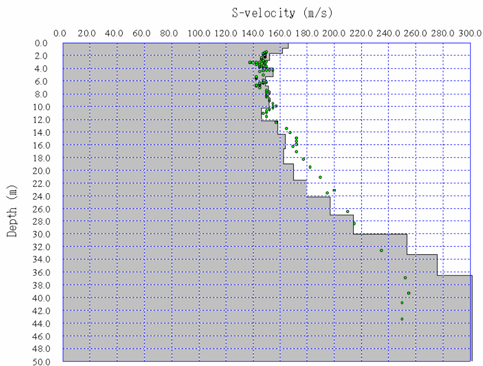
Figure 5.4.7 Resultant S-wave velocity model for the north site.
