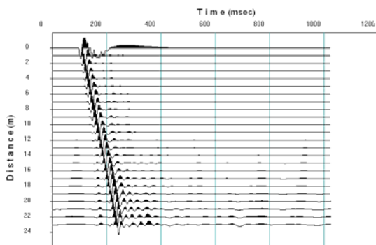
Land streamer
