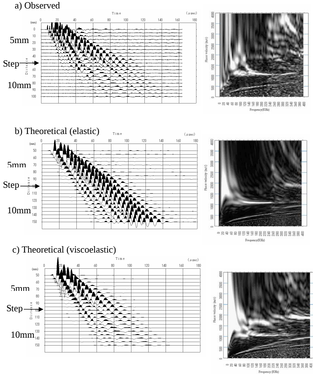
Figure 3.4.13. Comparison of observed and theoretical data for two-dimensional model. a) Observed data. b) Theoretical data calculated by finite-difference method. c) Theoretical data calculated by finite-difference method including viscoelastic attenuation. Quality factor ( Q ) is assumed to be 10 for first layer (acrylic) and 100 for second layer (mortar).
