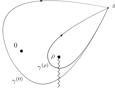
Figure 3 : Integration paths \gamma^{(0)} and \gamma^{(\rho)} .
