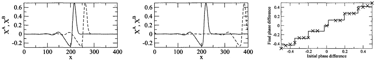
Figure 1: (Left, Middle) Multimodal phase locking between two pulses of coupled FitzHugh-Nagumo equations. (Right) Predicted steady phase shifts compared with the results of direct numerical simulations.
