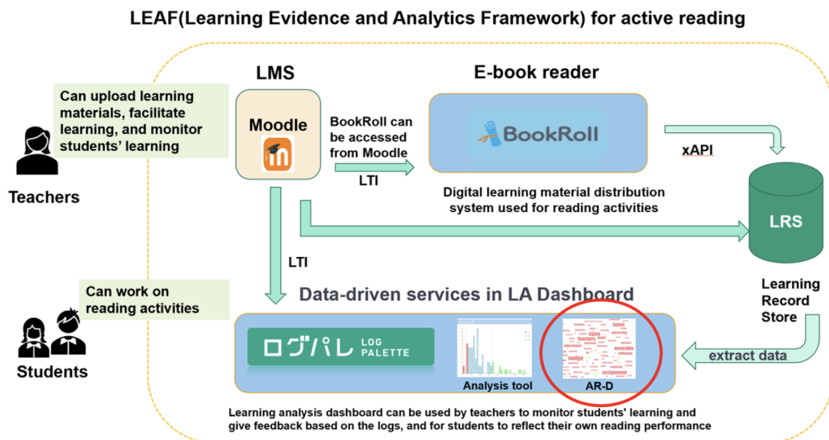
Figure 3.1: A framework of the LEAF system
